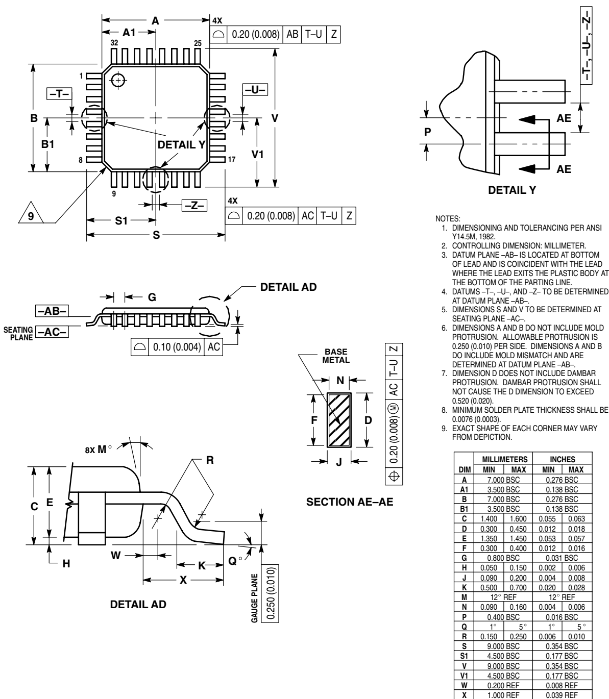
Figure 11-2 56F8023 32-Pin LQFP Mechanical Information
