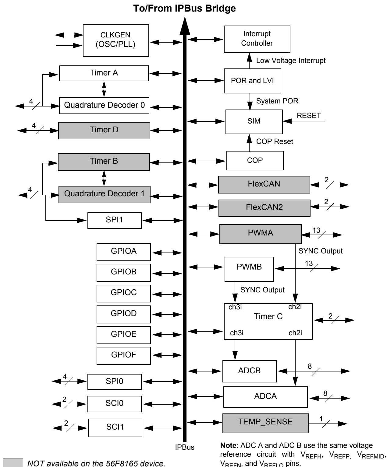
Figure 1-2 Peripheral Subsystem
