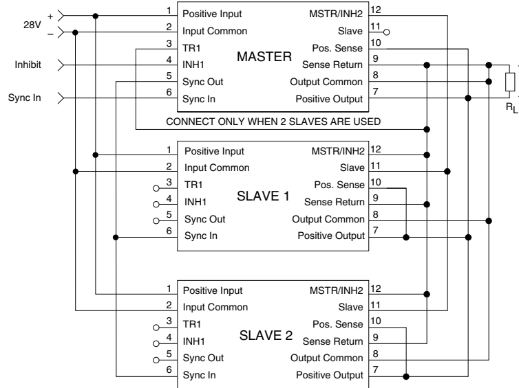
FIGURE 2: PARALLEL CONNECTIONS
