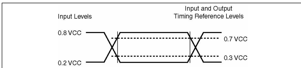
Figure 18. AC Measurement I/O Waveform
