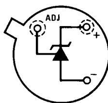
20139720 Bottom View See NS Package Number H03H
