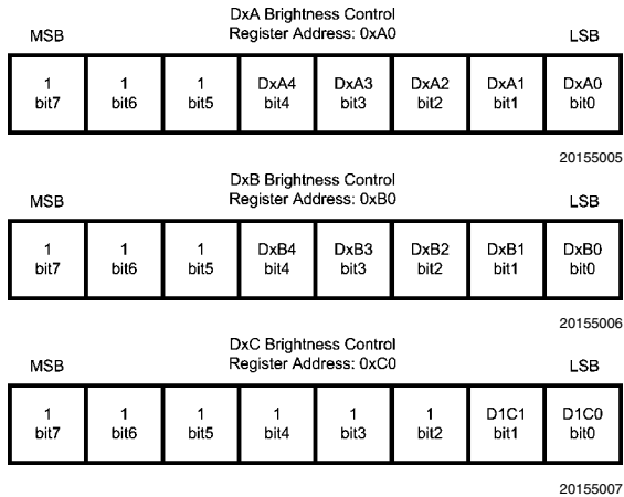
FIGURE 6. Brightness Control Register Description Internal Hex Address: 0xA0 (BankA), 0xB0 (BankB), 0xC0 (BankC)
