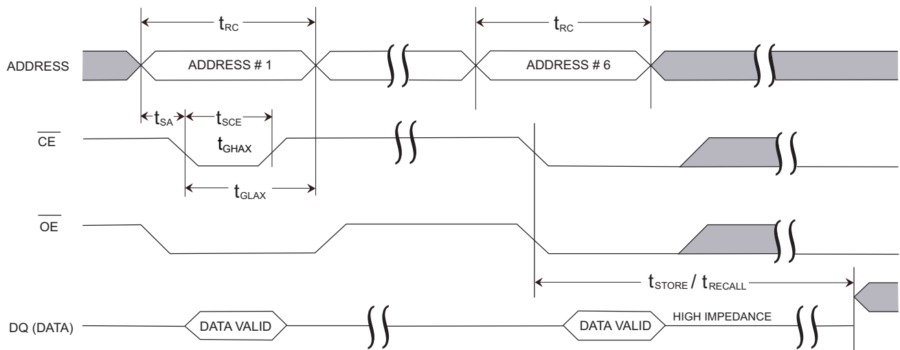
Figure 6. \overline{\text{CE}} -Controlled Software STORE/RECALL Cycle [19]
