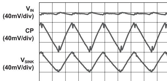
Load Characteristics ( V_{IN} = 3.1V ; 2X Mode; 20mA/Channel)
