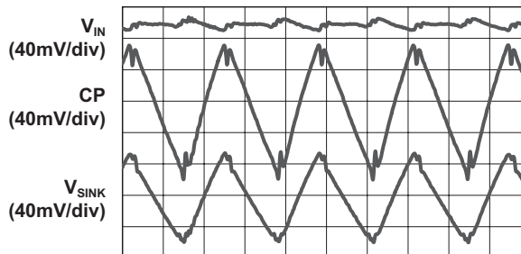
Load Characteristics ( V_{IN} = 3.6V ; 2X Mode; 30mA/Channel)
