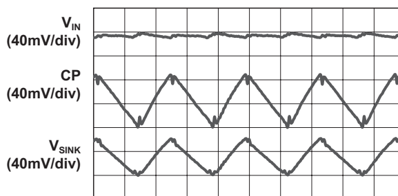
Load Characteristics ( V_{IN} = 2.9V ; 2X Mode; 15mA/Channel)
