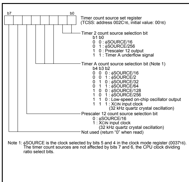
Fig 24. Structure of timer count source set register
