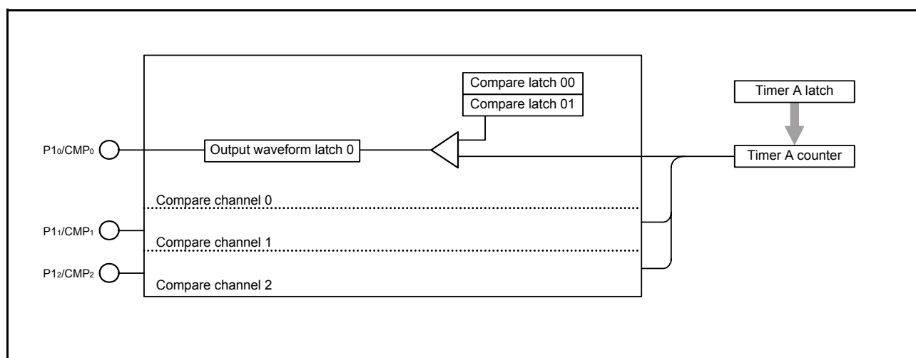
Fig 34. Block diagram of compare output circuit
