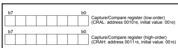
Fig 27. Structure of capture/compare register
