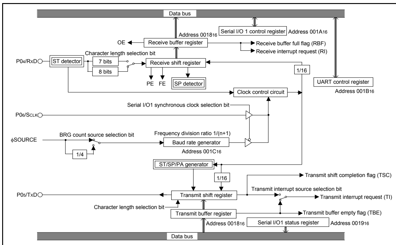
Fig 45. Block diagram of UART serial I/O
