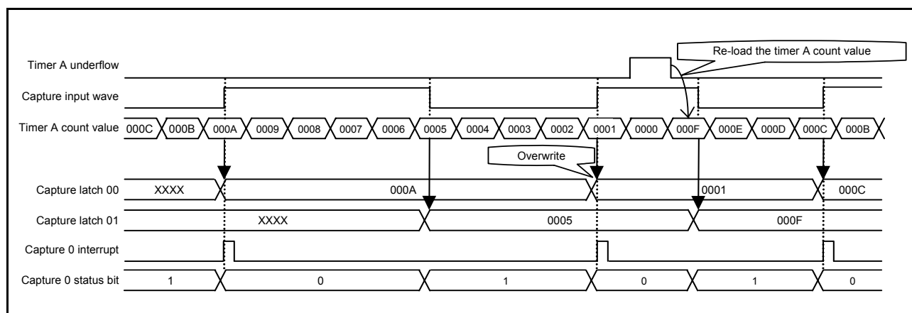
Fig 41. Capture input waveform (capture interrupt edge selection bit = “rising edge”)
