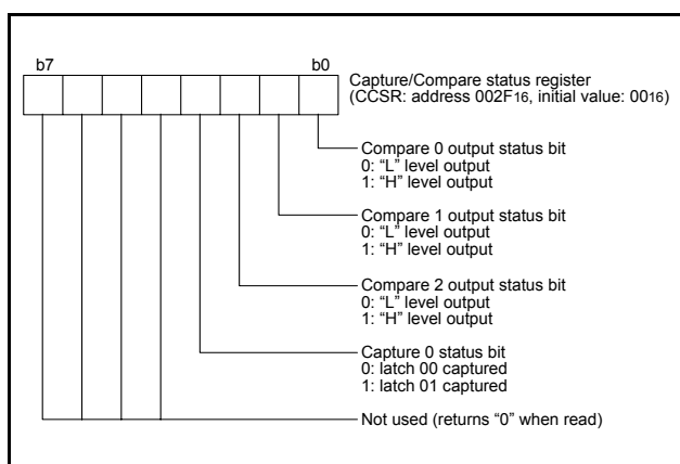
Fig 32. Structure of capture/compare status register
