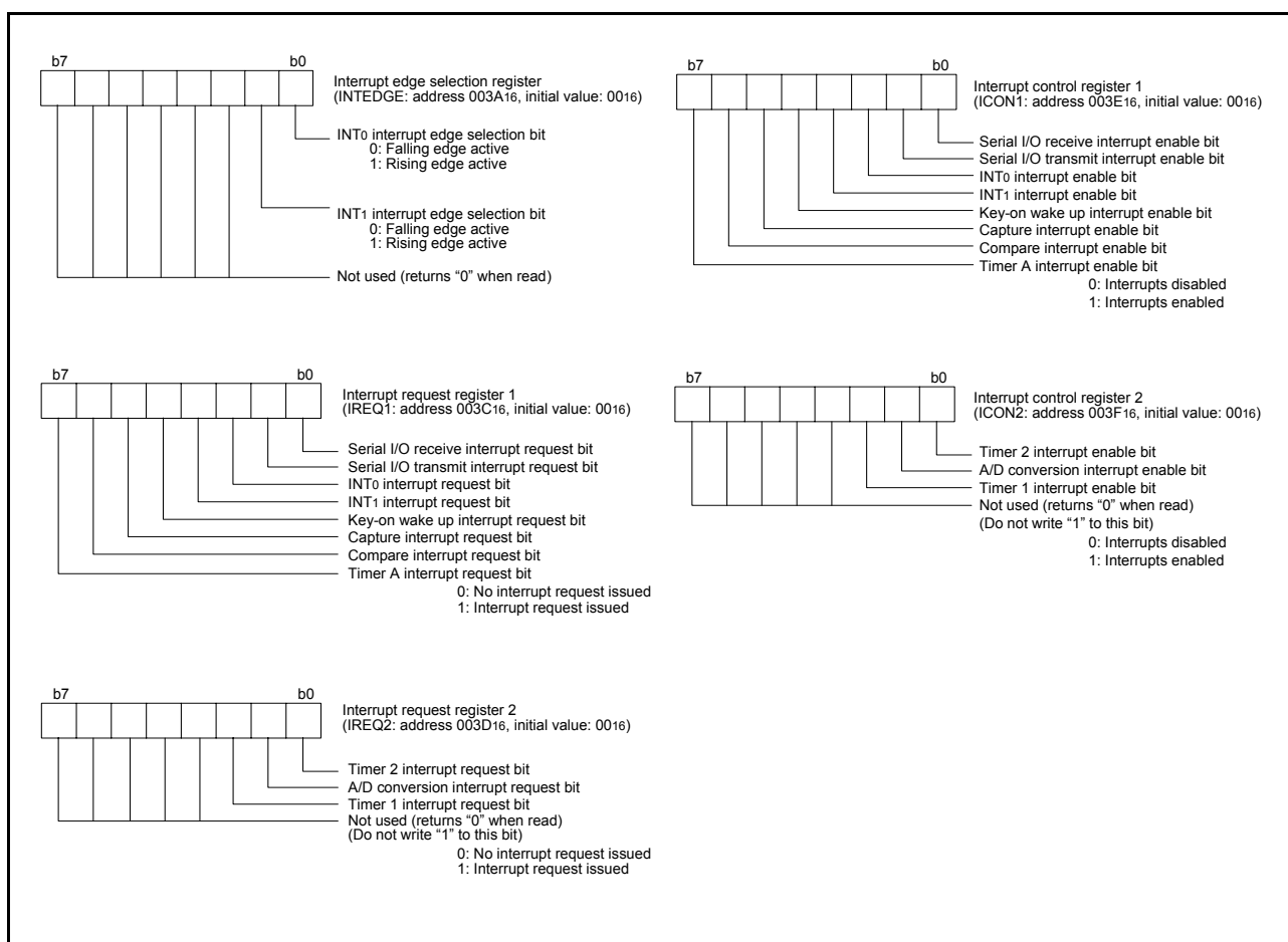
Fig 21. Structure of Interrupt-related registers
