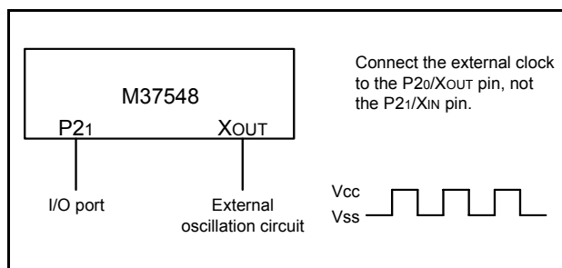
Fig 61. External clock input circuit
