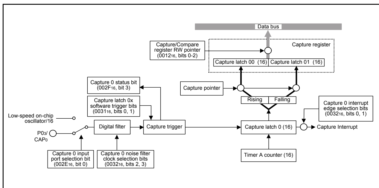
Fig 40. Block diagram of capture channel 0
