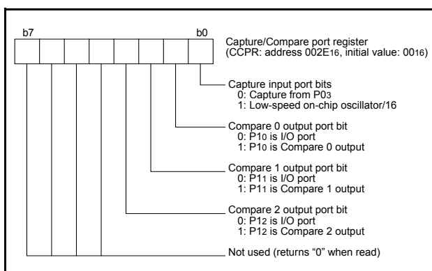
Fig 30. Structure of capture/compare port register
