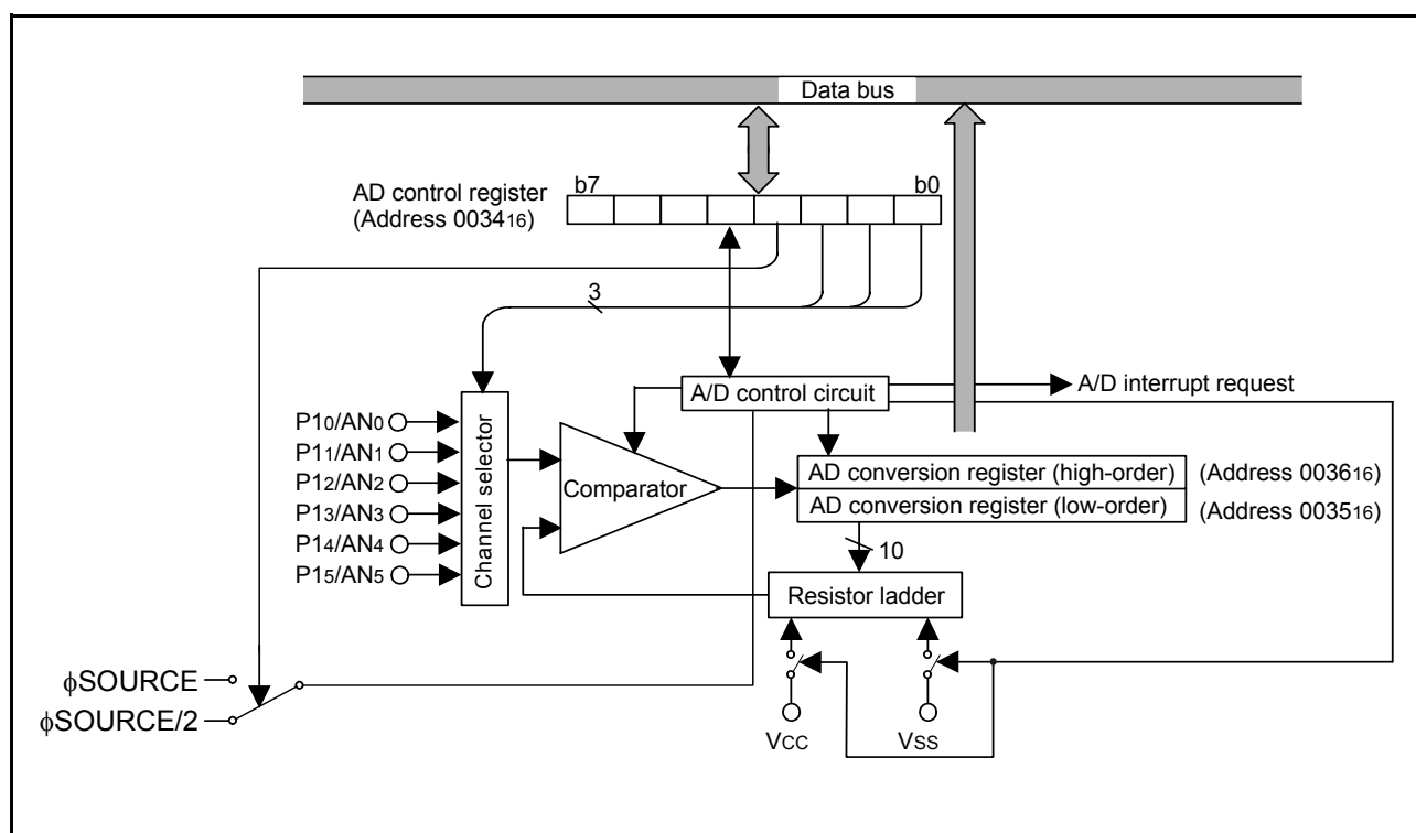
Fig 50. Block diagram of A/D converter
