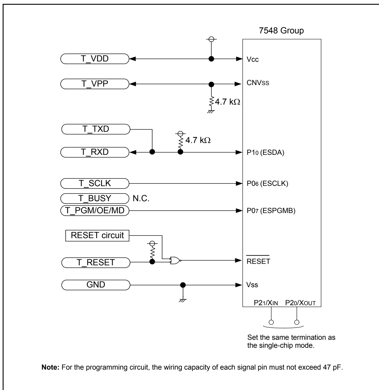
Fig 69. When using programmer of Suisai Electronics System Co., LTD, connection example
