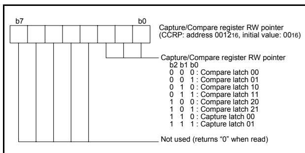
Fig 28. Structure of capture/compare register RW pointer
