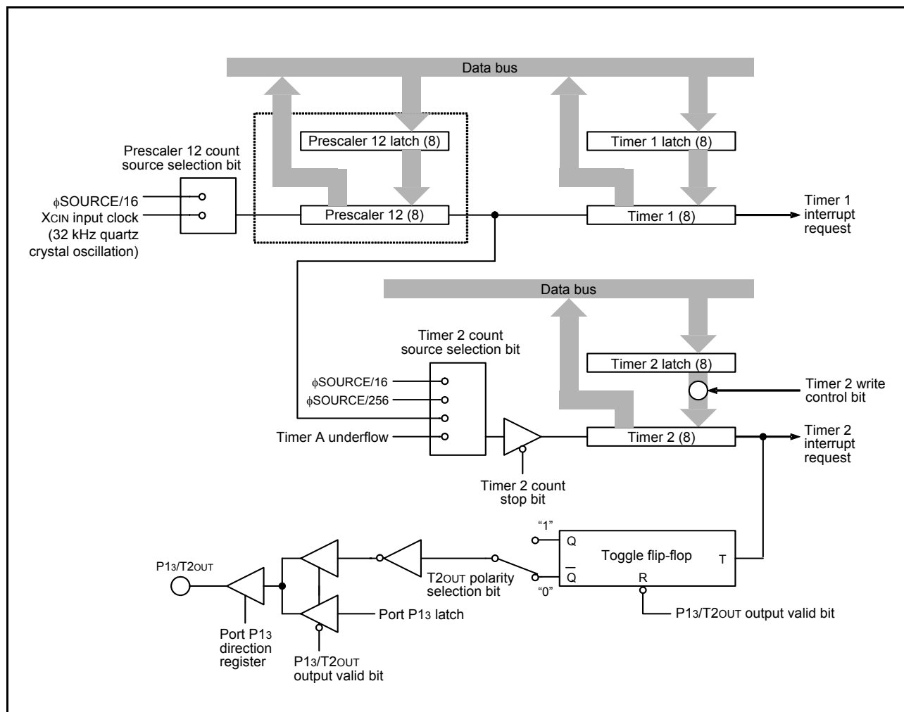
Fig 25. Block diagram of timer 1 and timer 2
