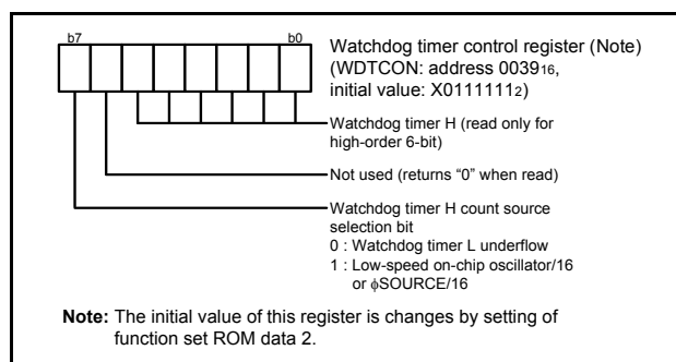
Fig 52. Structure of watchdog timer control register
