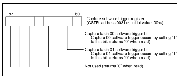
Fig 38. Structure of capture software trigger register
