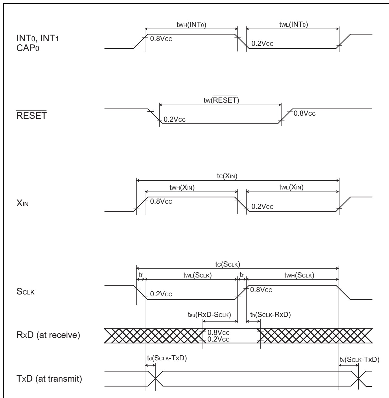
Fig 84. Timing chart
