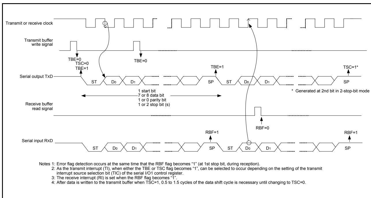
Fig 46. Operation of UART serial I/O function
