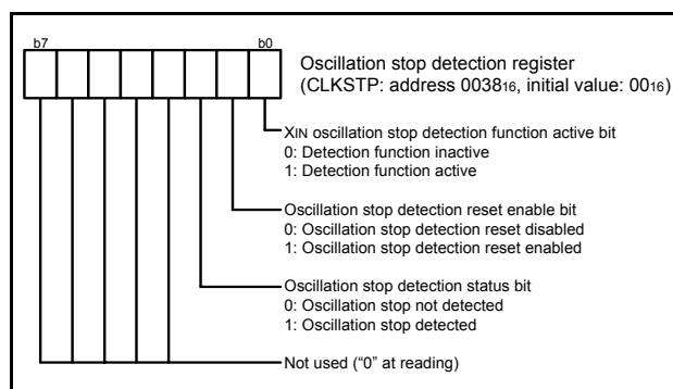
Fig 65. Structure of oscillation stop detection register
