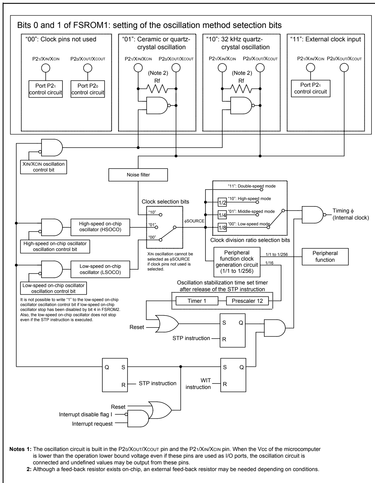
Fig 63. Block diagram of internal clock generating circuit
