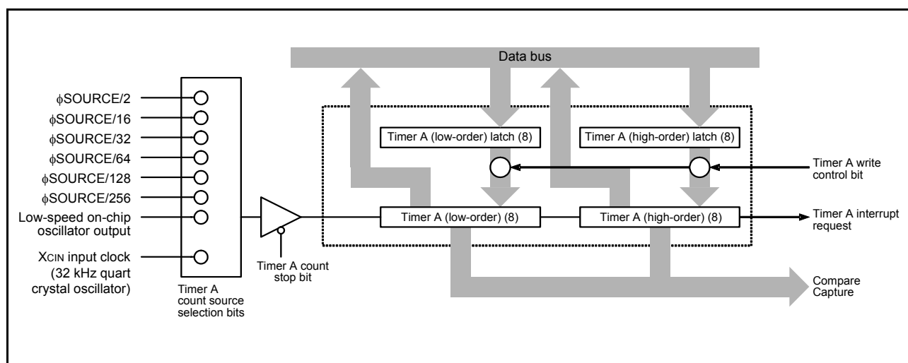
Fig 26. Block diagram of timer A
