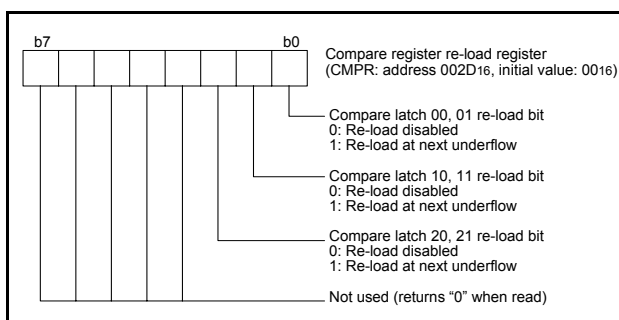
Fig 29. Structure of compare register re-load register
