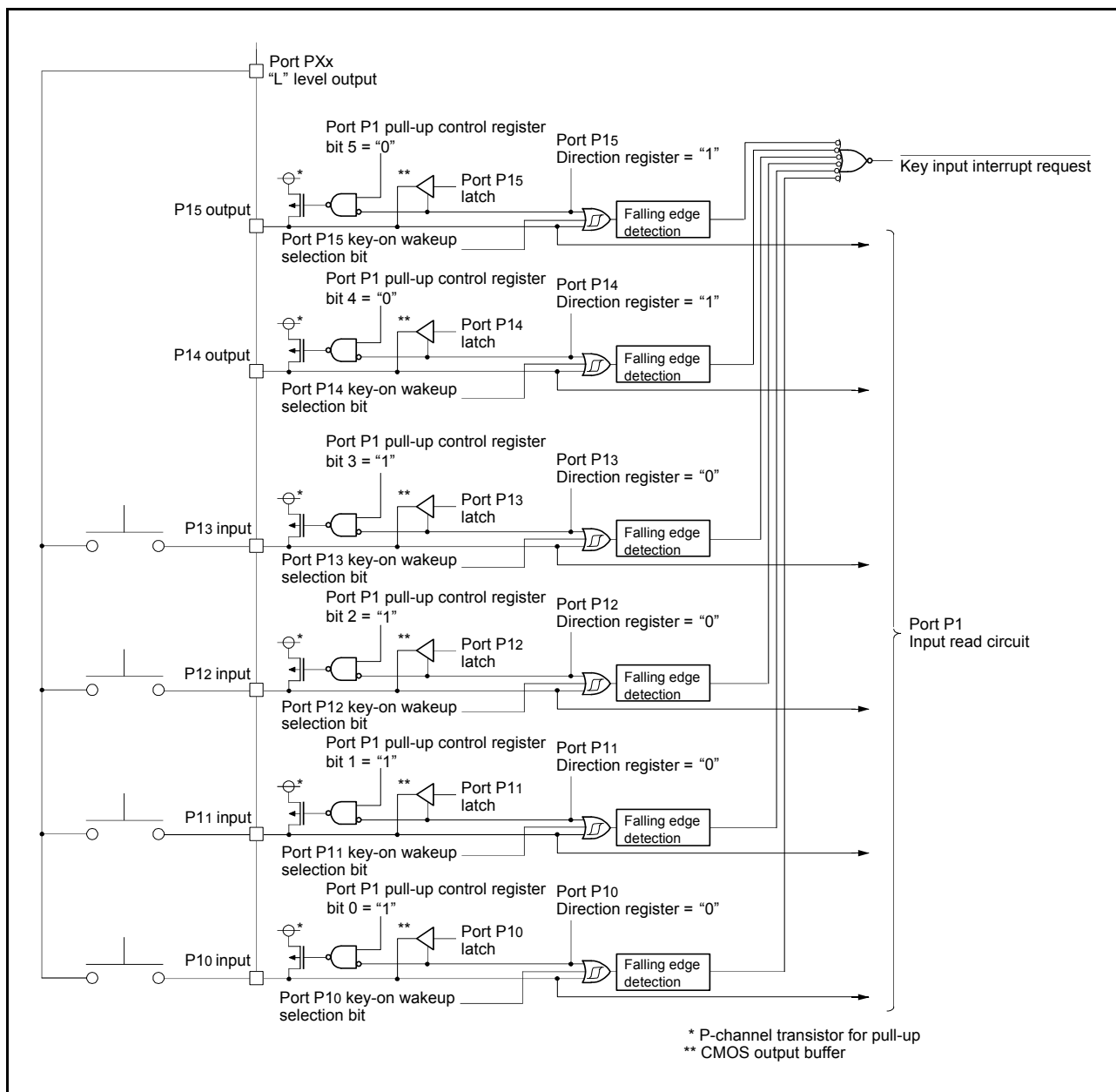
Fig 22. Connection example when using key input interrupt and port P1 block diagram
