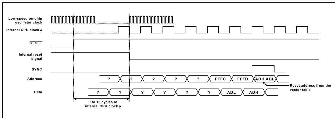
Fig 56. Timing diagram at reset
