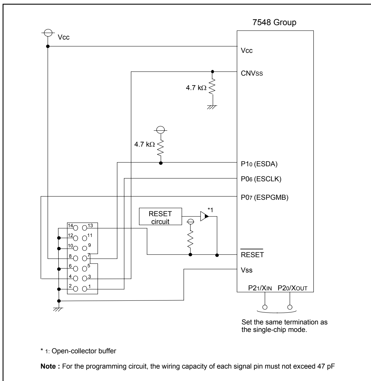
Fig 68. When using E8 programmer, connection example
