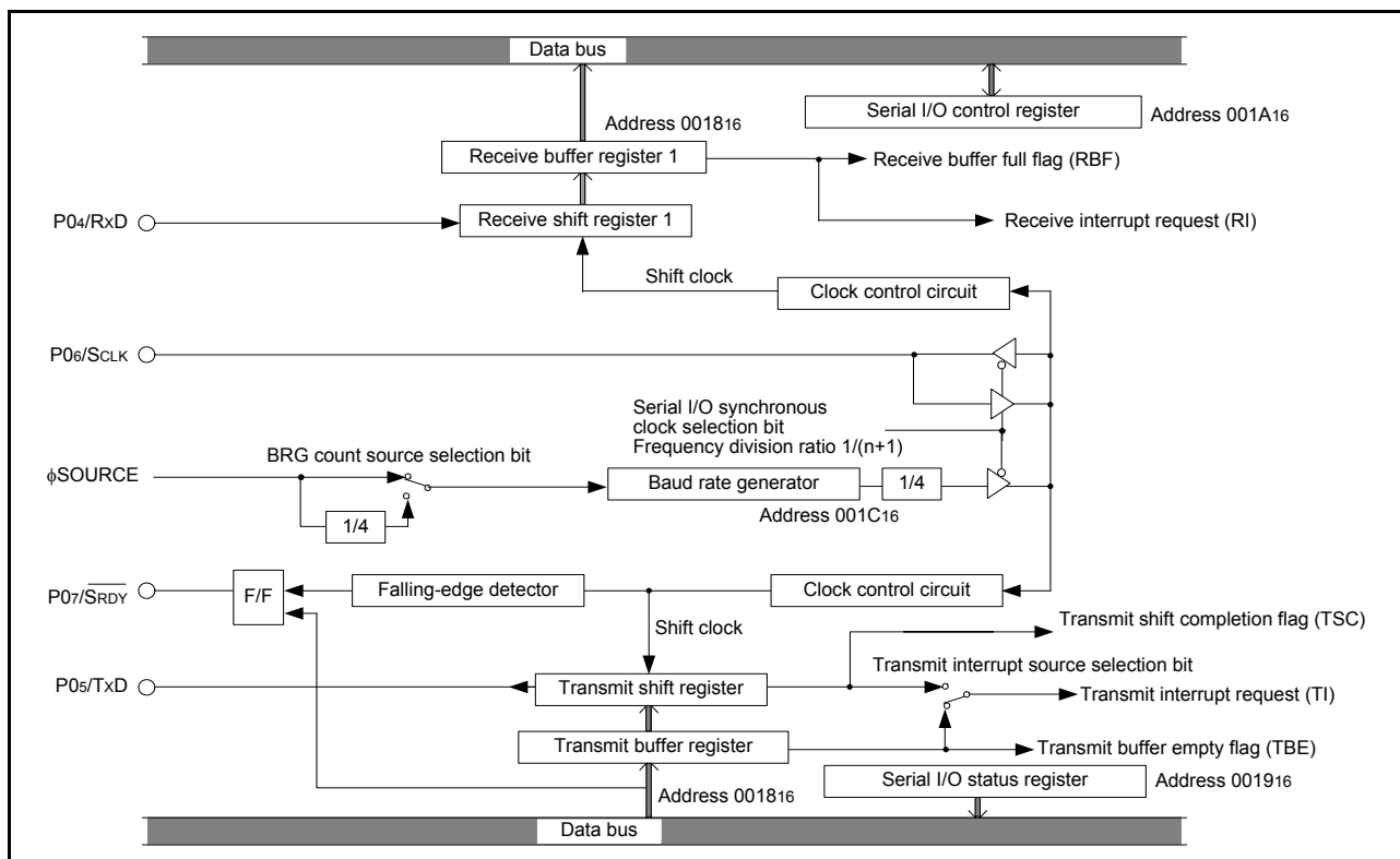
Fig 43. Block diagram of clock synchronous serial I/O
