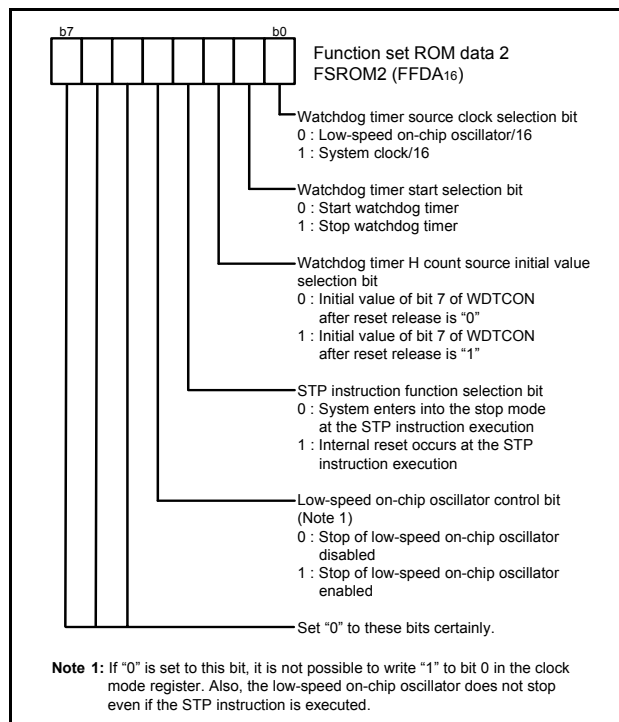
Fig 51. Structure of Function set ROM data 2
