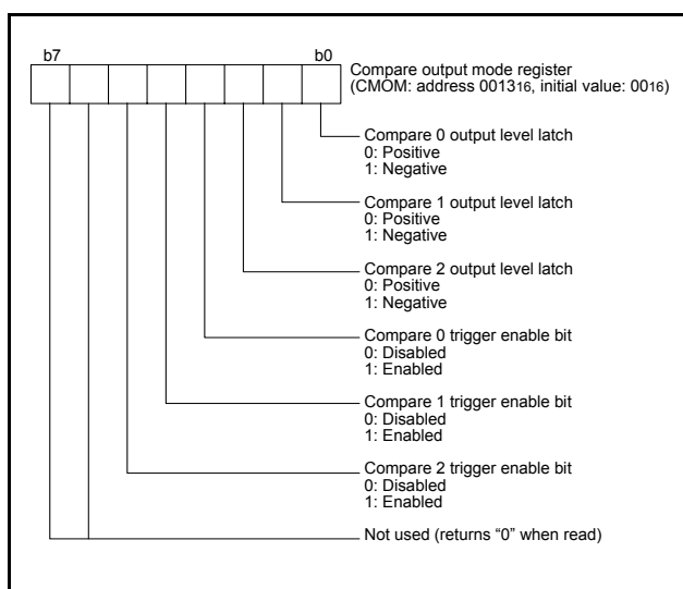
Fig 31. Structure of compare output mode register
