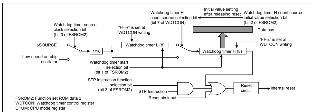
Fig 53. Block diagram of watchdog timer
