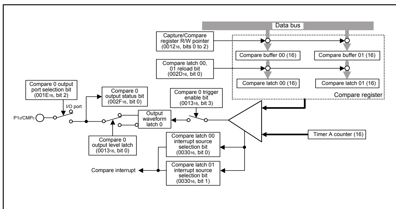
Fig 35. Block diagram of compare channel 0
