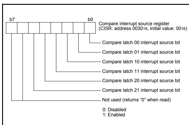
Fig 33. Structure of compare interrupt source register
