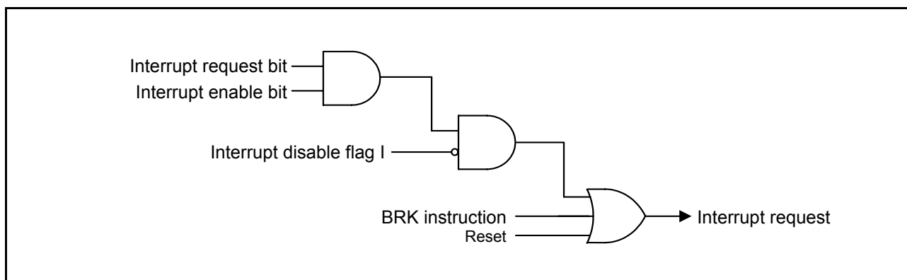
Fig 20. Interrupt control
