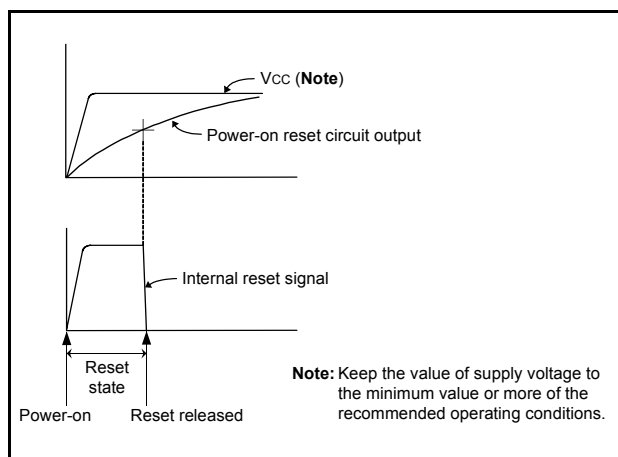
Fig 54. Operation waveform diagram of power-on reset circuit
