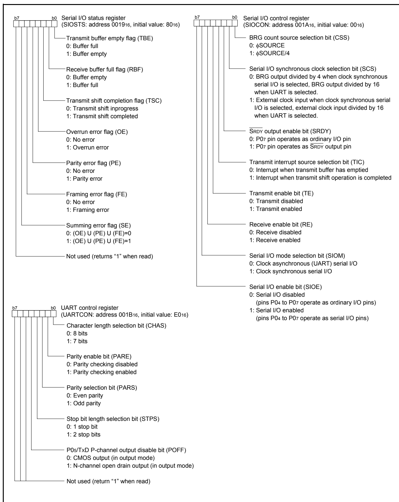
Fig 47. Structure of serial I/O1-related registers
