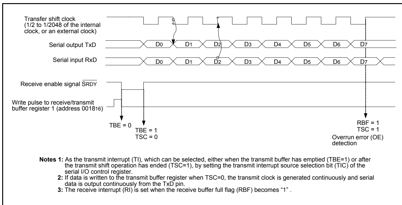
Fig 44. Operation of clock synchronous serial I/O function
