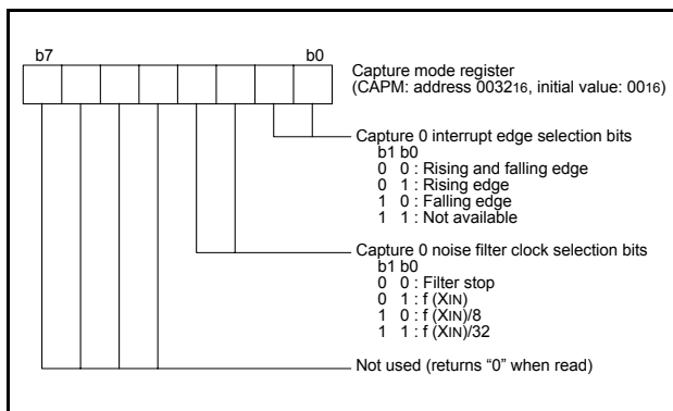
Fig 39. Structure of capture mode register
