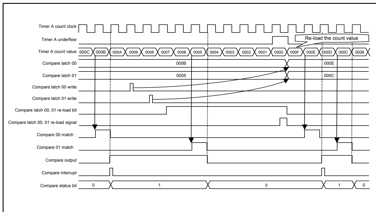
Fig 37. Output compare mode (compare register write timing)
