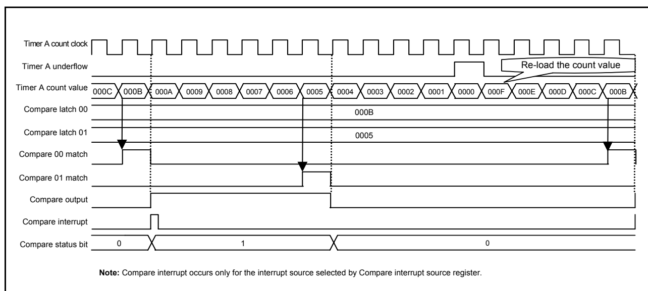
Fig 36. Output compare mode (general waveform)
