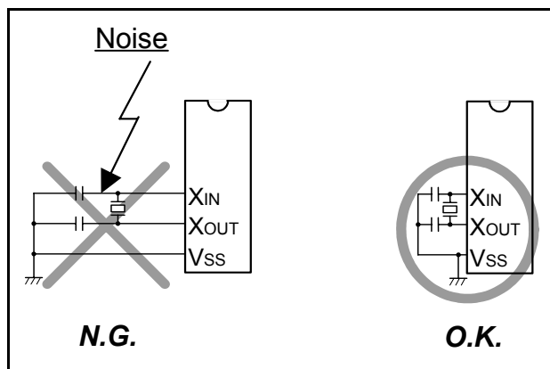
Fig 72. Wiring for clock I/O pins
