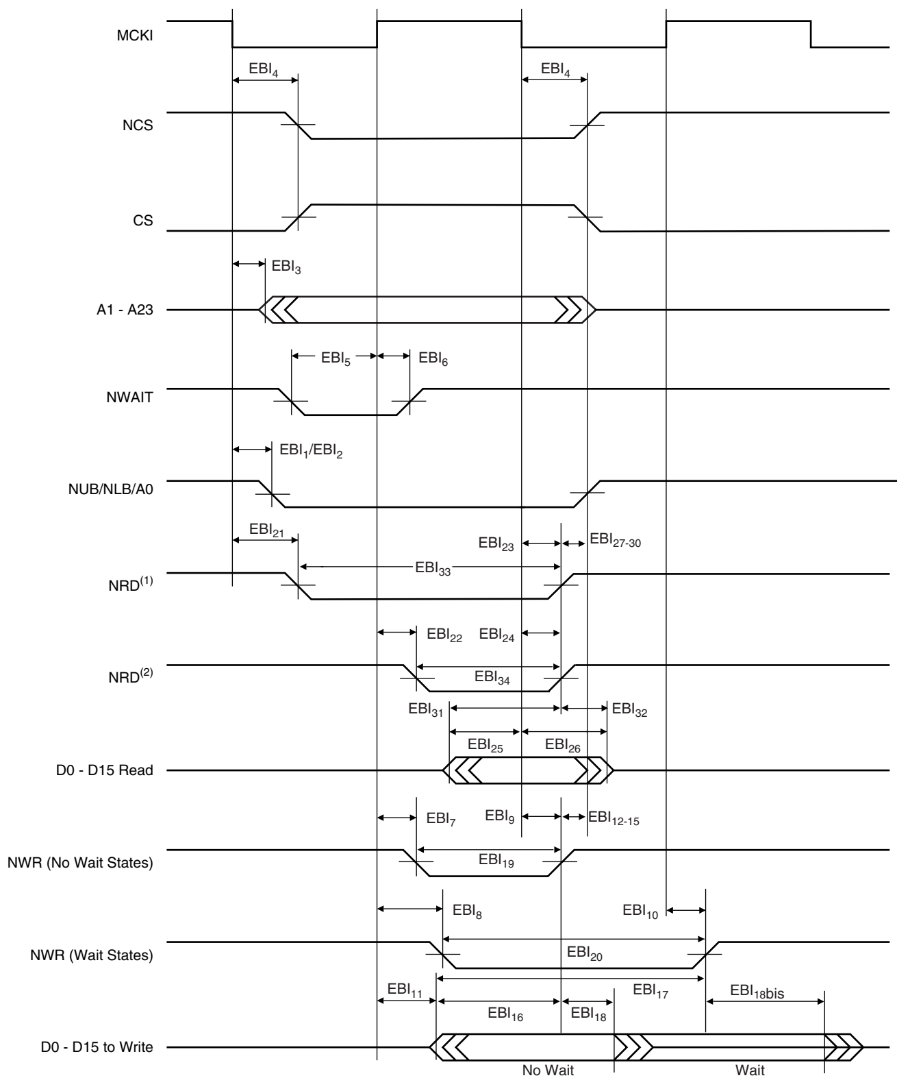
Figure 21-10. EBI Signals Relative to MCKI
