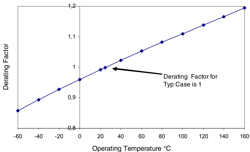
Figure 21-1. Derating Curve for Different Operating Temperatures
