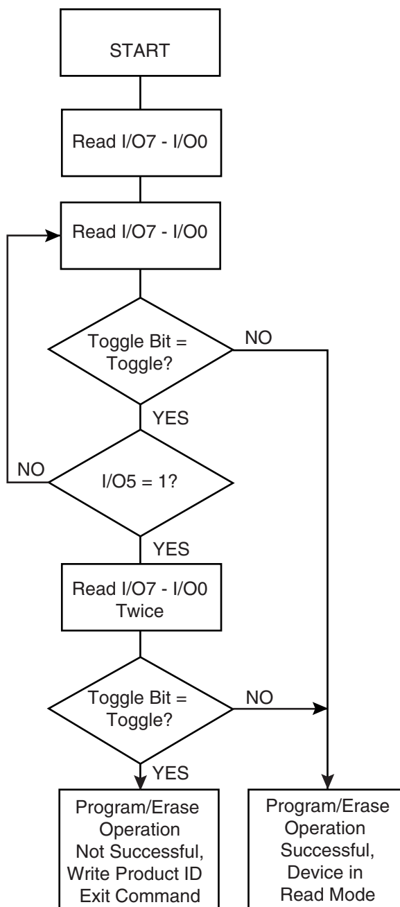
Figure 12-4. Toggle Bit Algorithm (Configuration Register = 00)
