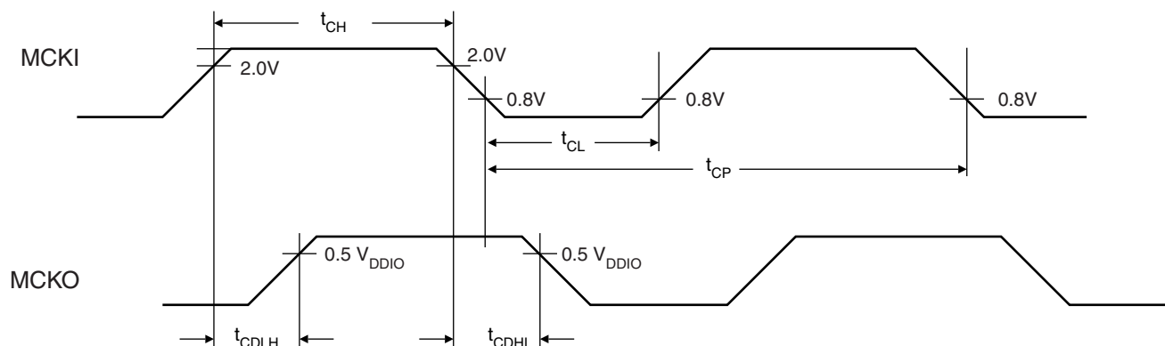
Figure 20-1. Clock Waveform
