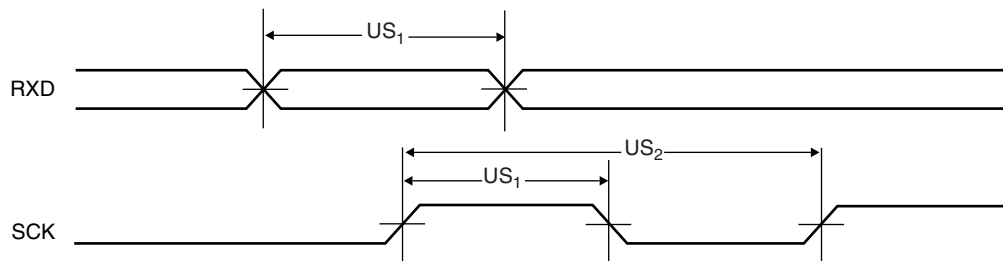
Figure 21-4. USART Signals
