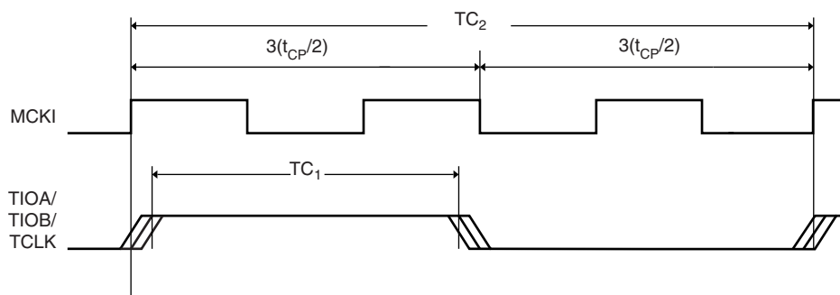
Figure 21-5. Timer Input
