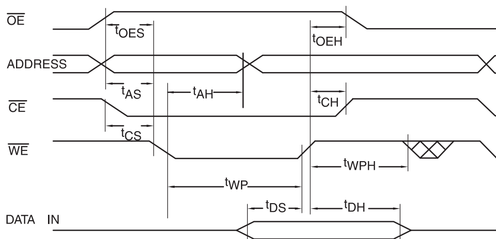
Figure 21-14. \overline{WE} Controlled
