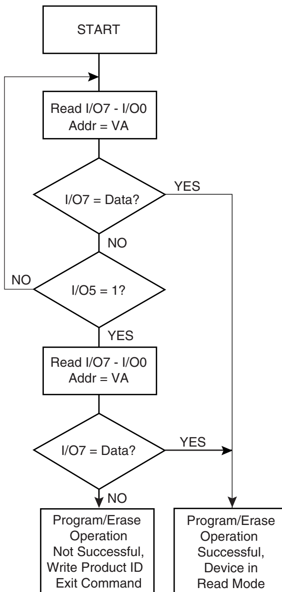
Figure 12-2. Data Polling Algorithm (Configuration Register = 00)
