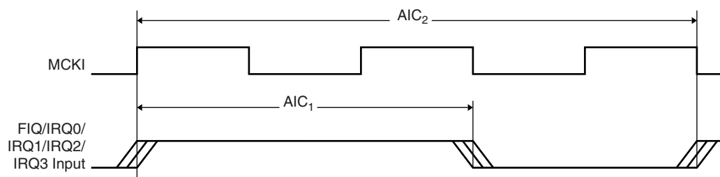
Figure 21-7. AIC Signals
