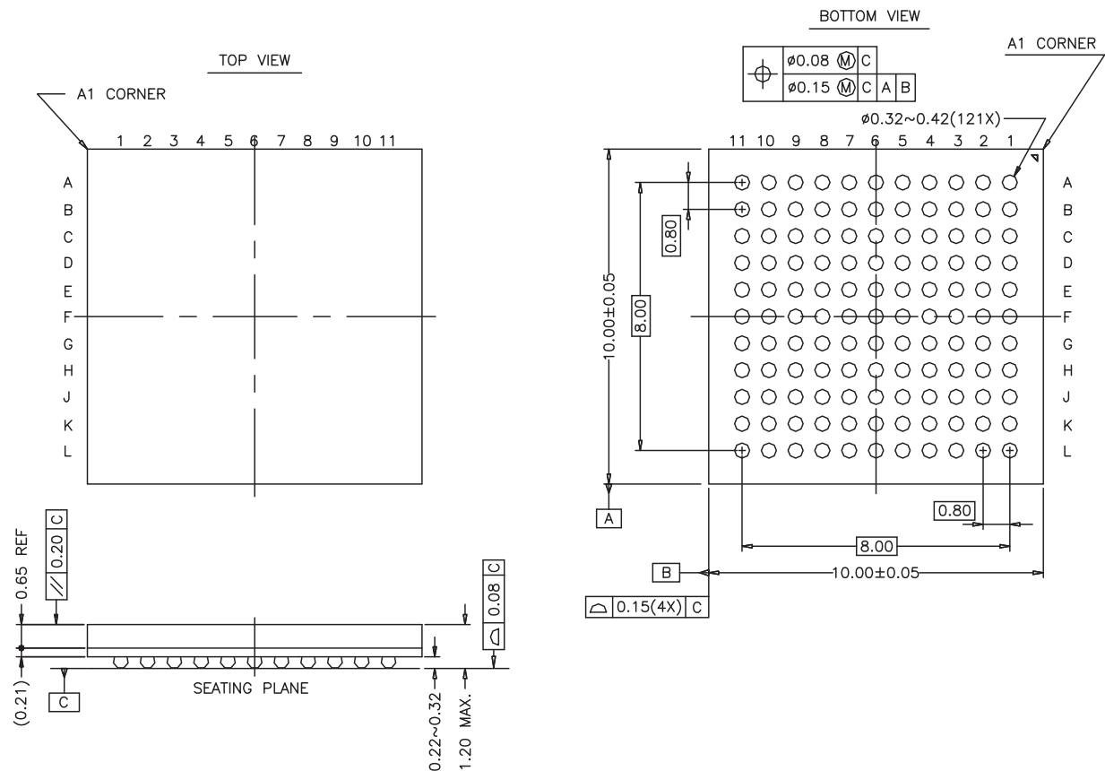
Figure 22-1. AT91FR40162SB Package
