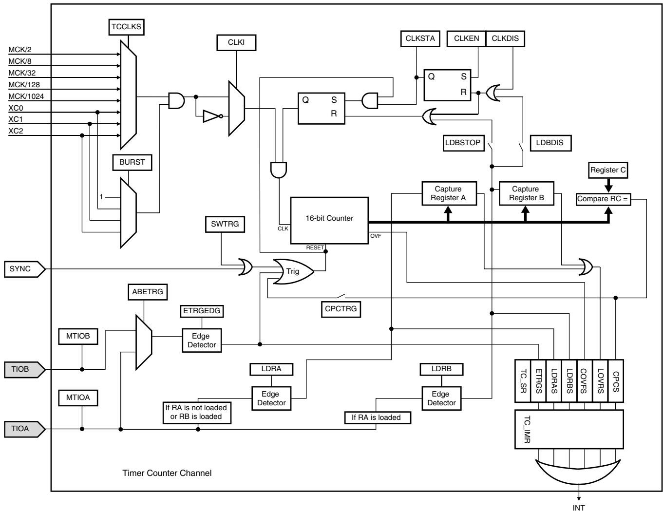
Figure 19-4. Capture Mode
