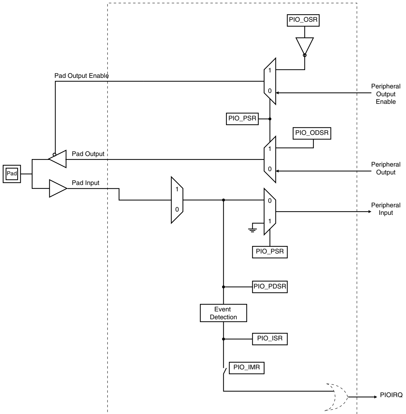
Figure 15-1. Parallel I/O Multiplexed with a Bi-directional Signal
