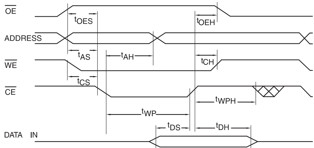
Figure 21-15. CE Controlled
