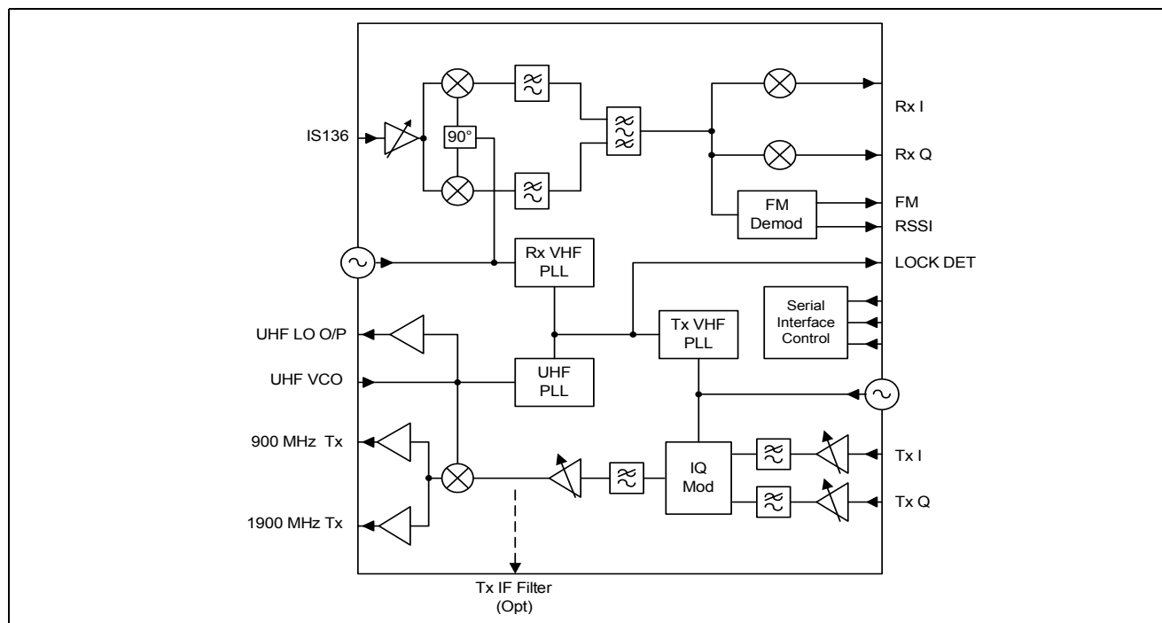
Figure 1 - Block Diagram
