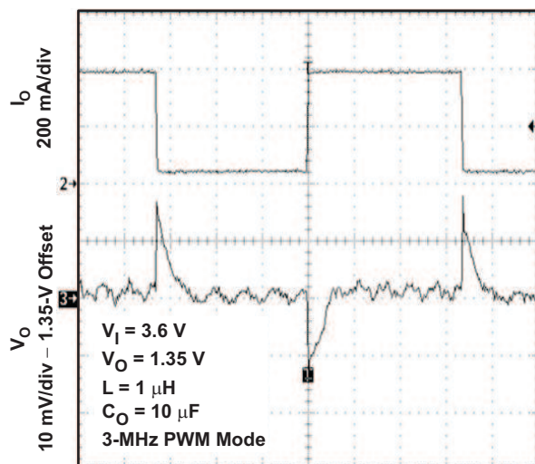
LOAD TRANSIENT: 50 mA / 400 mA / 50 mA PWM OPERATION
