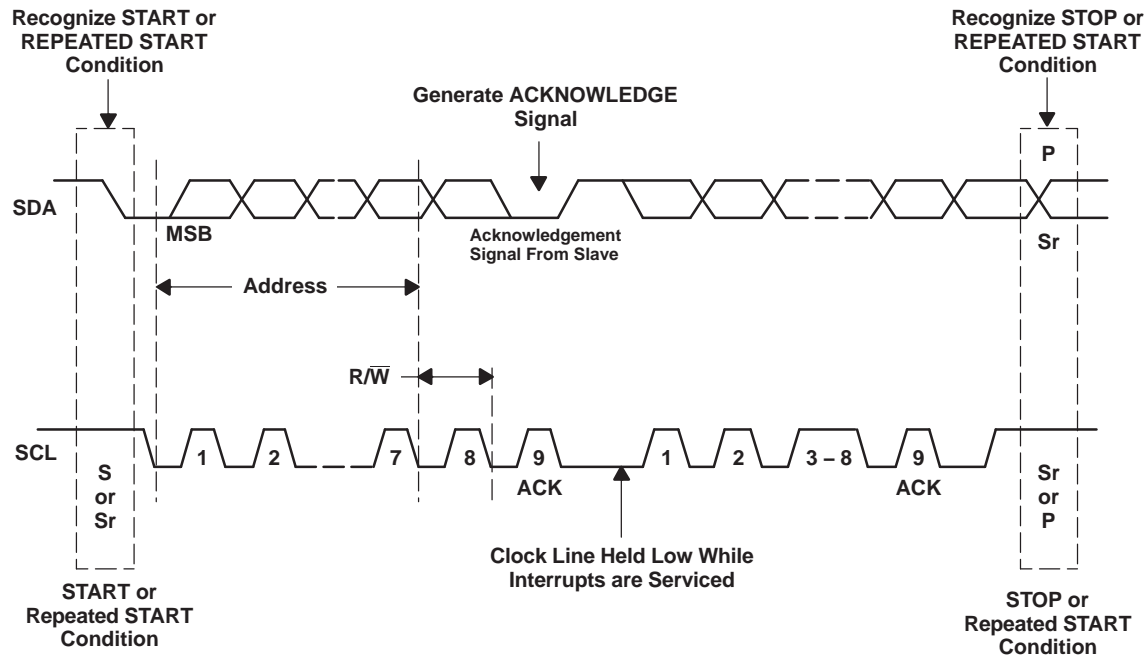
Figure 48. Bus Protocol
