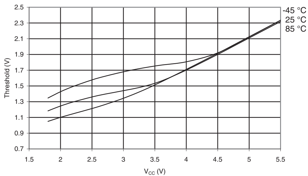
Figure 29-37. Reset Input Threshold Voltage vs. V_{CC} ( V_{IH,Reset} Pin Read as “1”)
