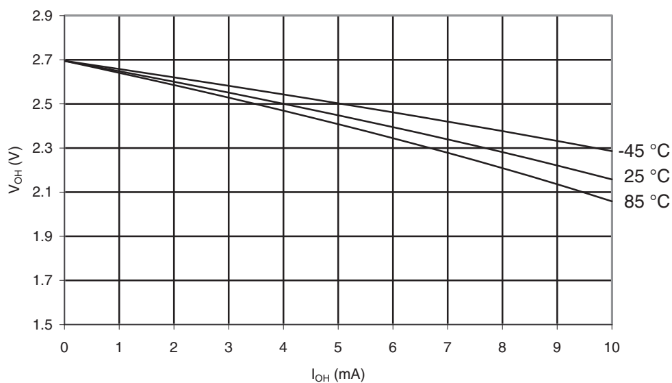
Figure 29-23. I/O Pin Output Voltage vs. Source Current, Ports A, C, D, E, F, G ( V_{CC} = 2.7V )
