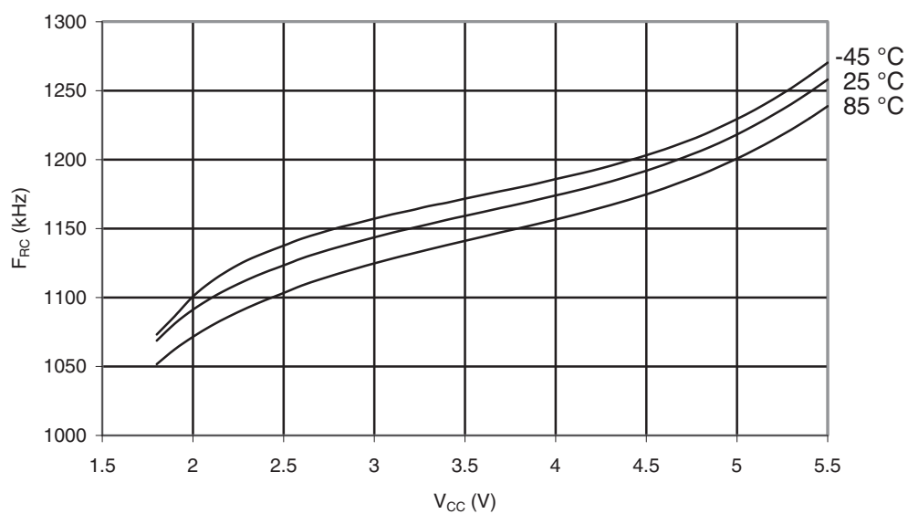
Figure 29-47. Watchdog Oscillator Frequency vs. V_{CC}
