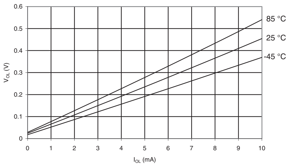
Figure 29-28. I/O Pin Output Voltage vs. Sink Current, Ports A, C, D, E, F, G ( V_{CC} = 5V )
