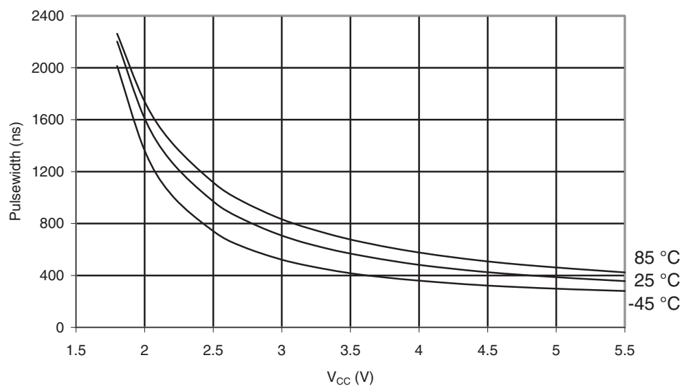
Figure 29-62. Minimum Reset Pulse Width vs. V_{CC}
