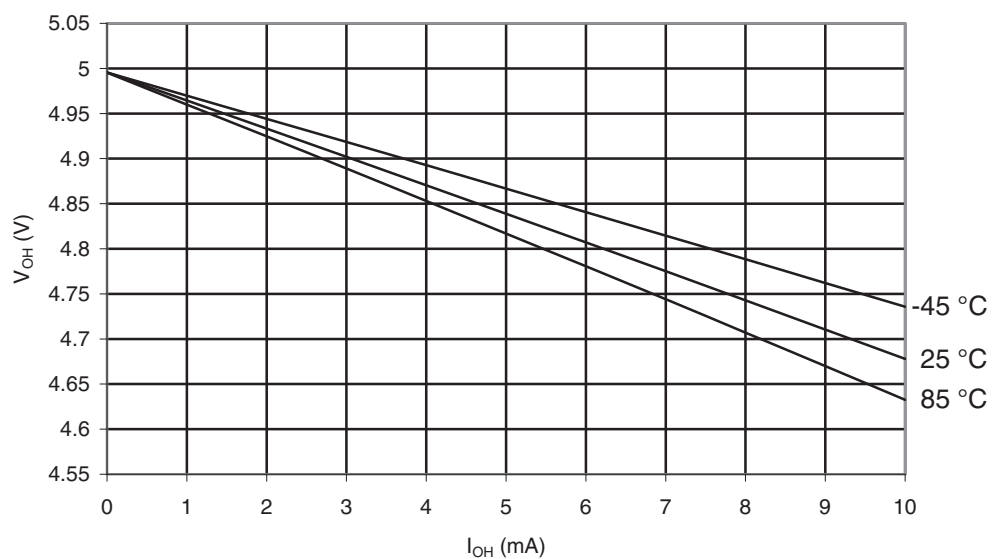
Figure 29-22. I/O Pin Output Voltage vs. Source Current, Ports A, C, D, E, F, G ( V_{CC} = 5V )
