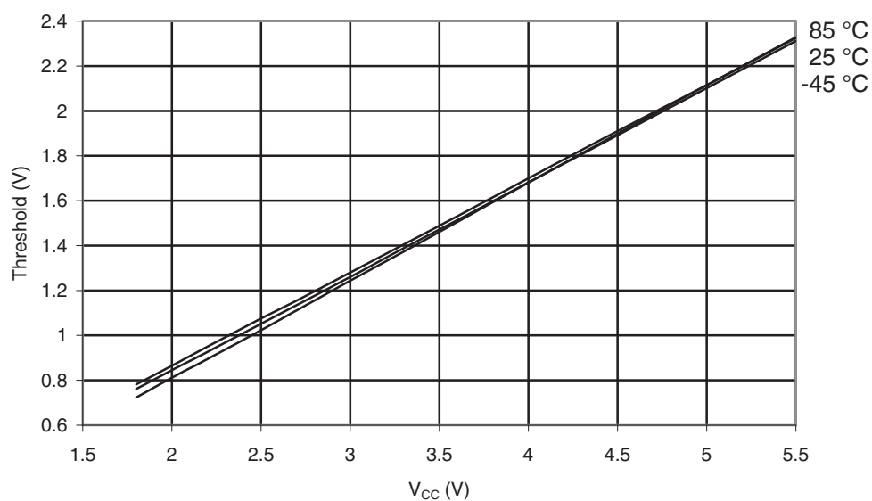
Figure 29-38. Reset Input Threshold Voltage vs. V_{CC} ( V_{IL} , Reset Pin Read as “0”)
