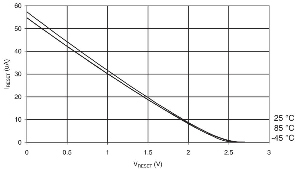
Figure 29-20. Reset Pull-up Resistor Current vs. Reset Pin Voltage ( V_{CC} = 2.7V )
