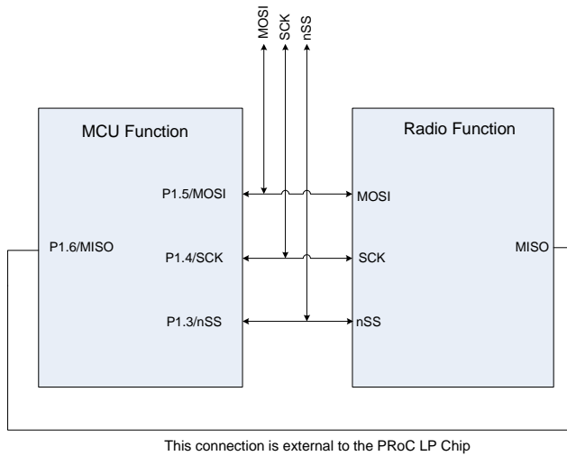
Figure 7. 4-Wire SPI Mode
