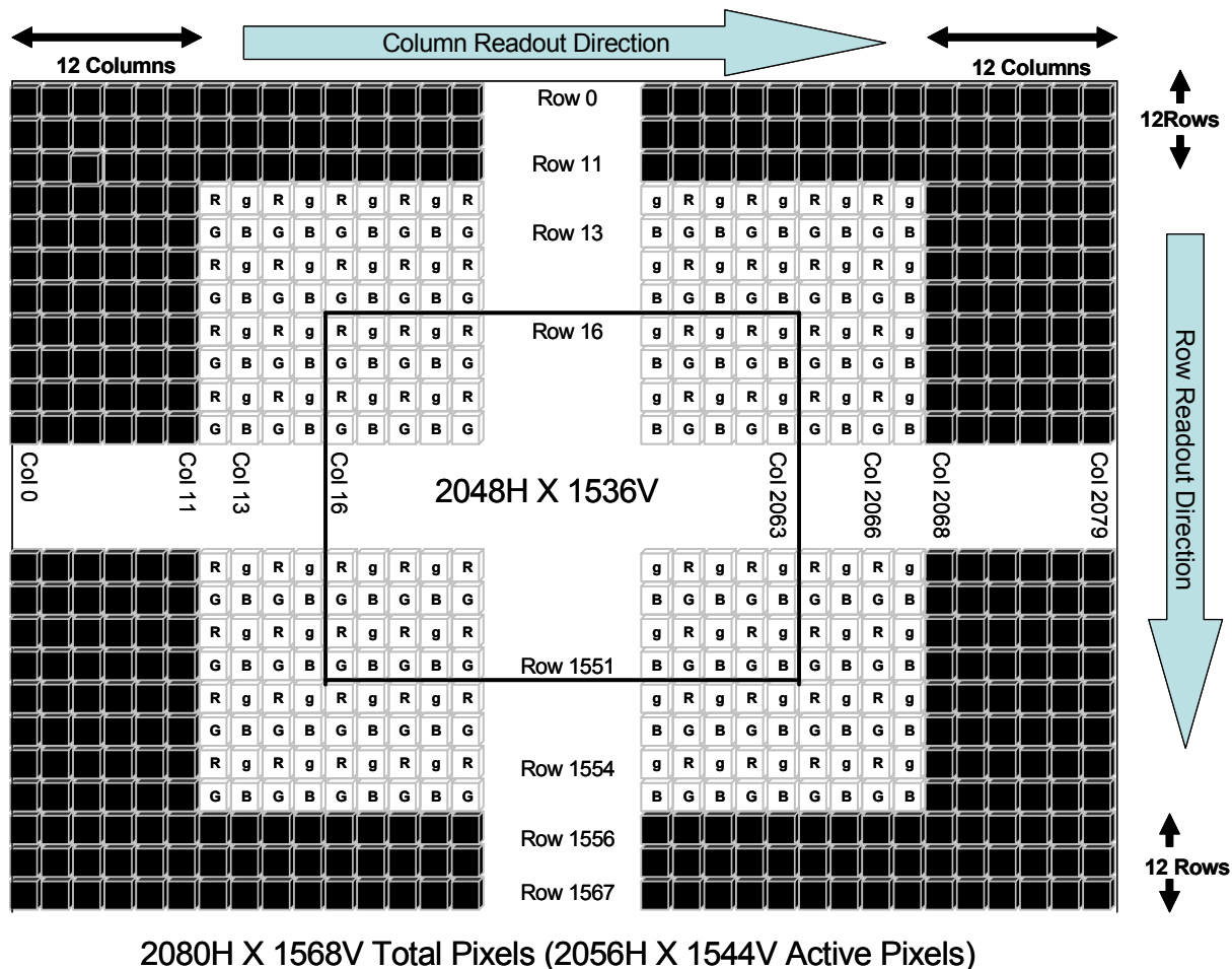
Figure 5-1. Pixel Array
