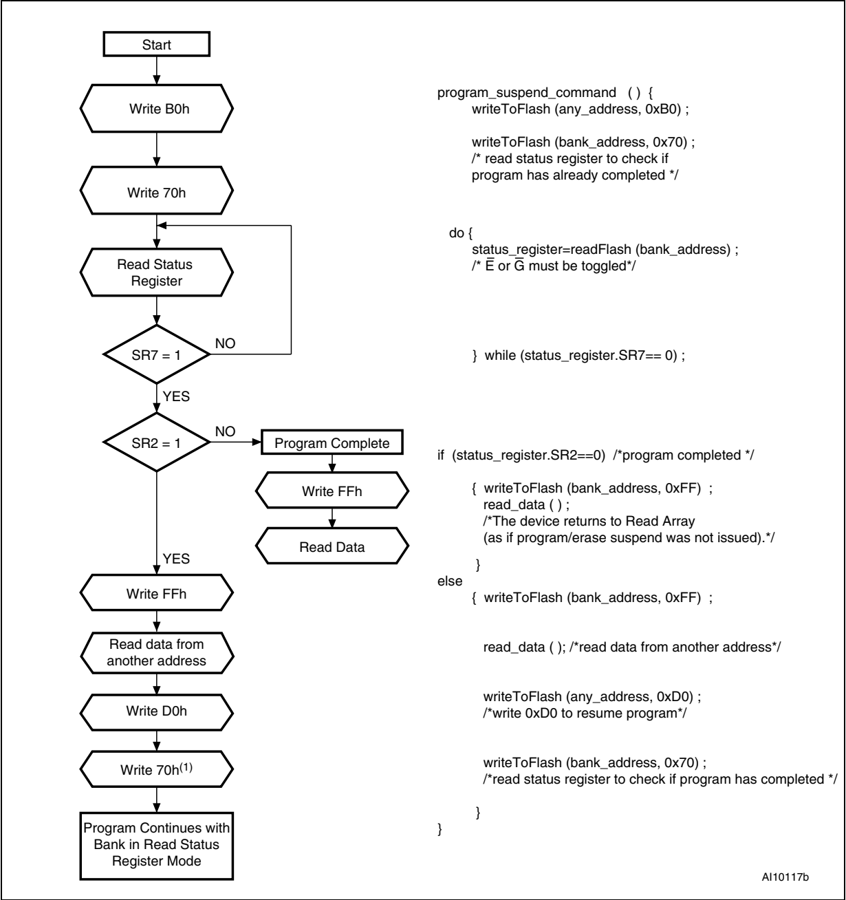
Figure 21. Program suspend and resume flowchart and pseudocode
