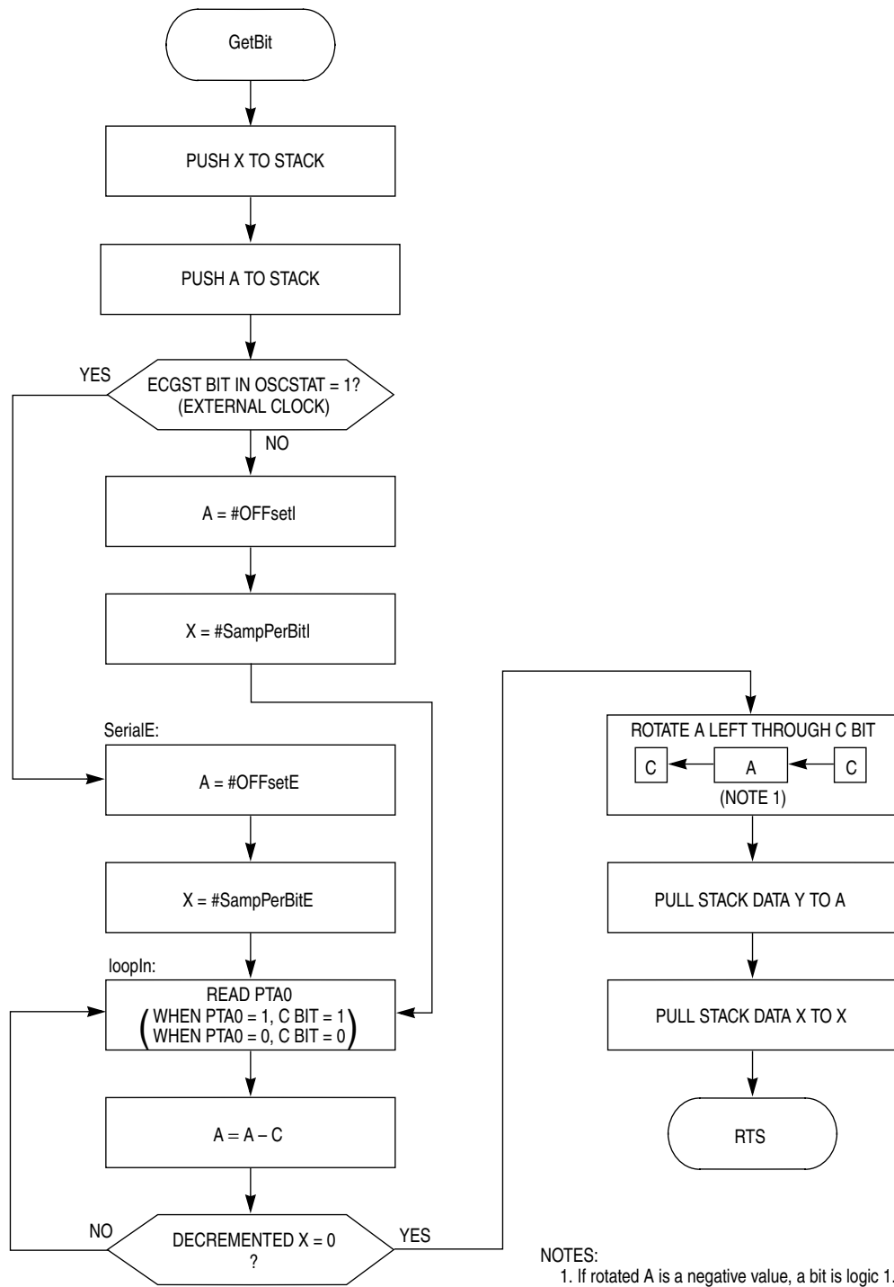
Figure 2. GetBit Routine
