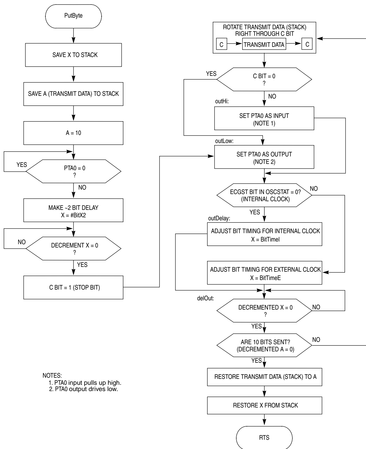
Figure 3. PutByte Routine
