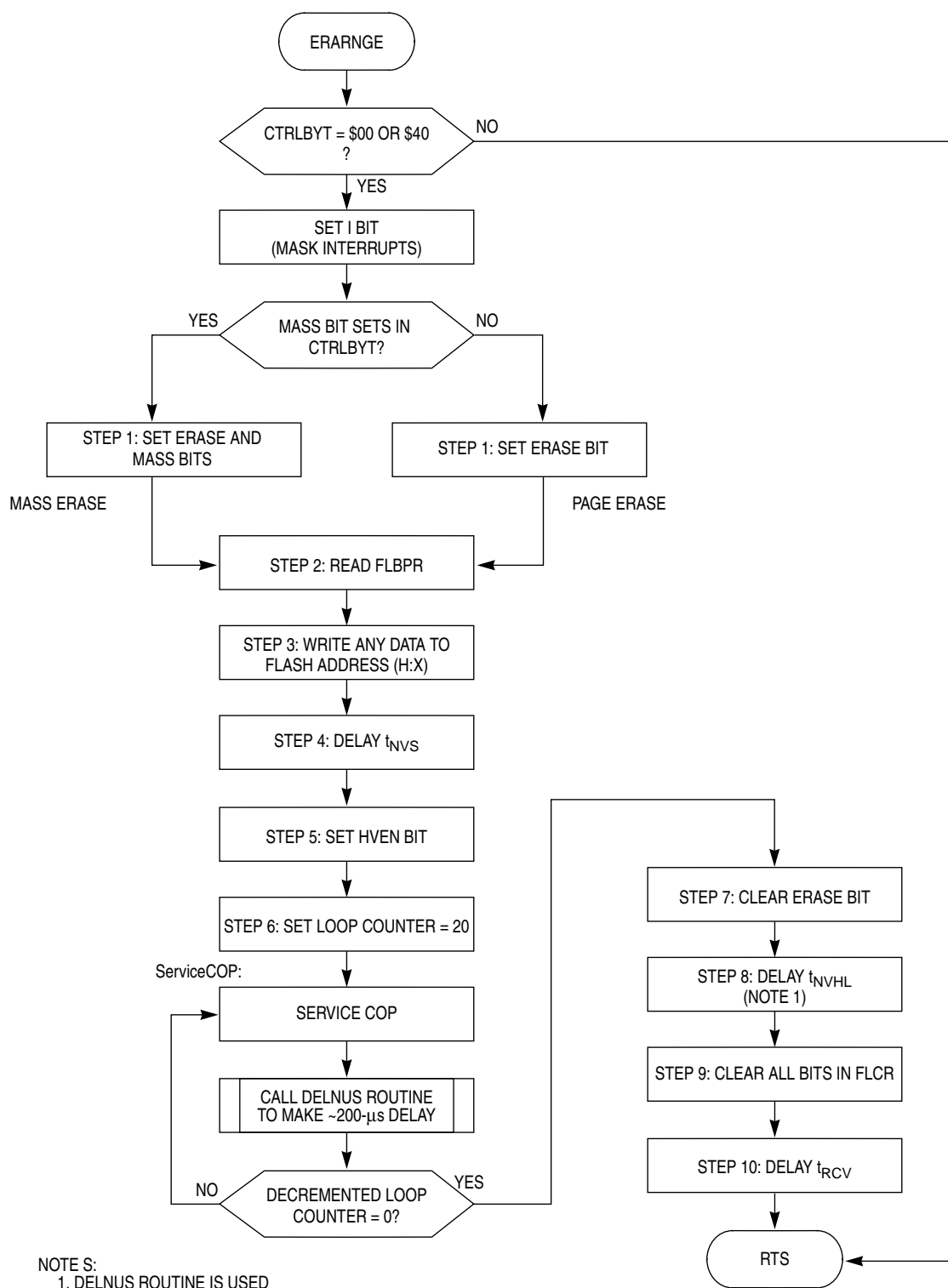
Figure 7. ERARNGE Routine
