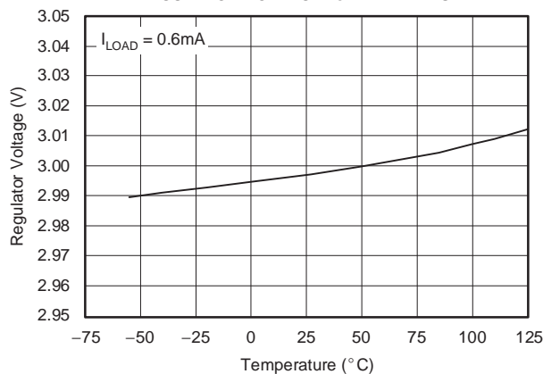
REGULATOR VOLTAGE vs TEMPERATURE
