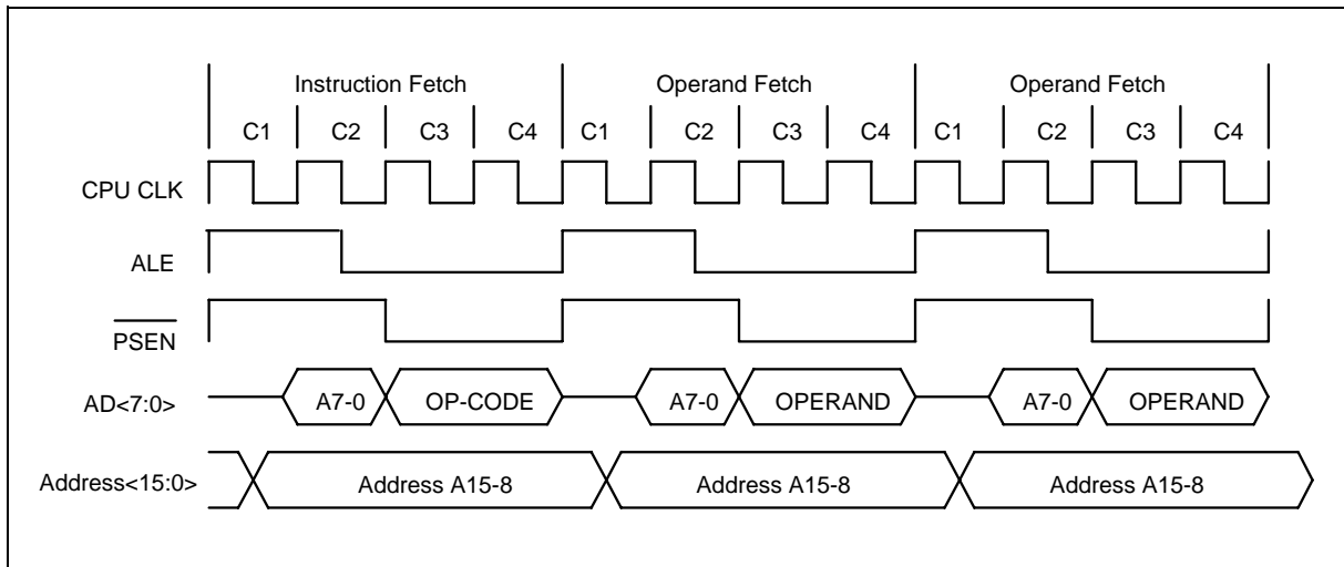
Figure 9-3: Three Cycles Instruction Timing
