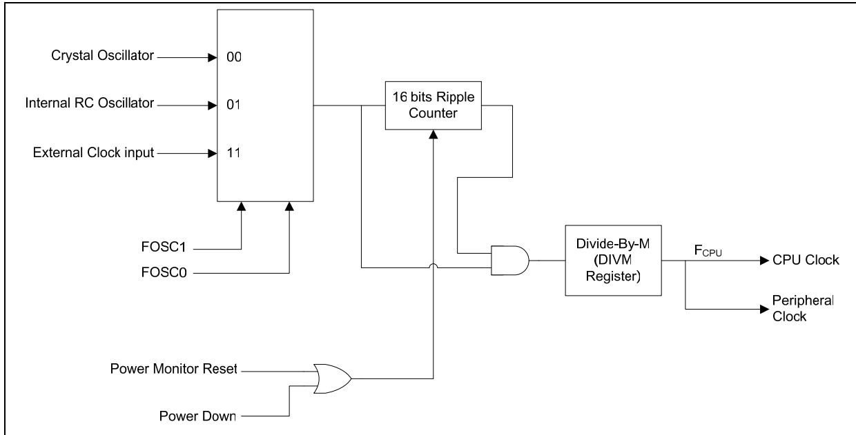
Figure 21-1: Oscillator
