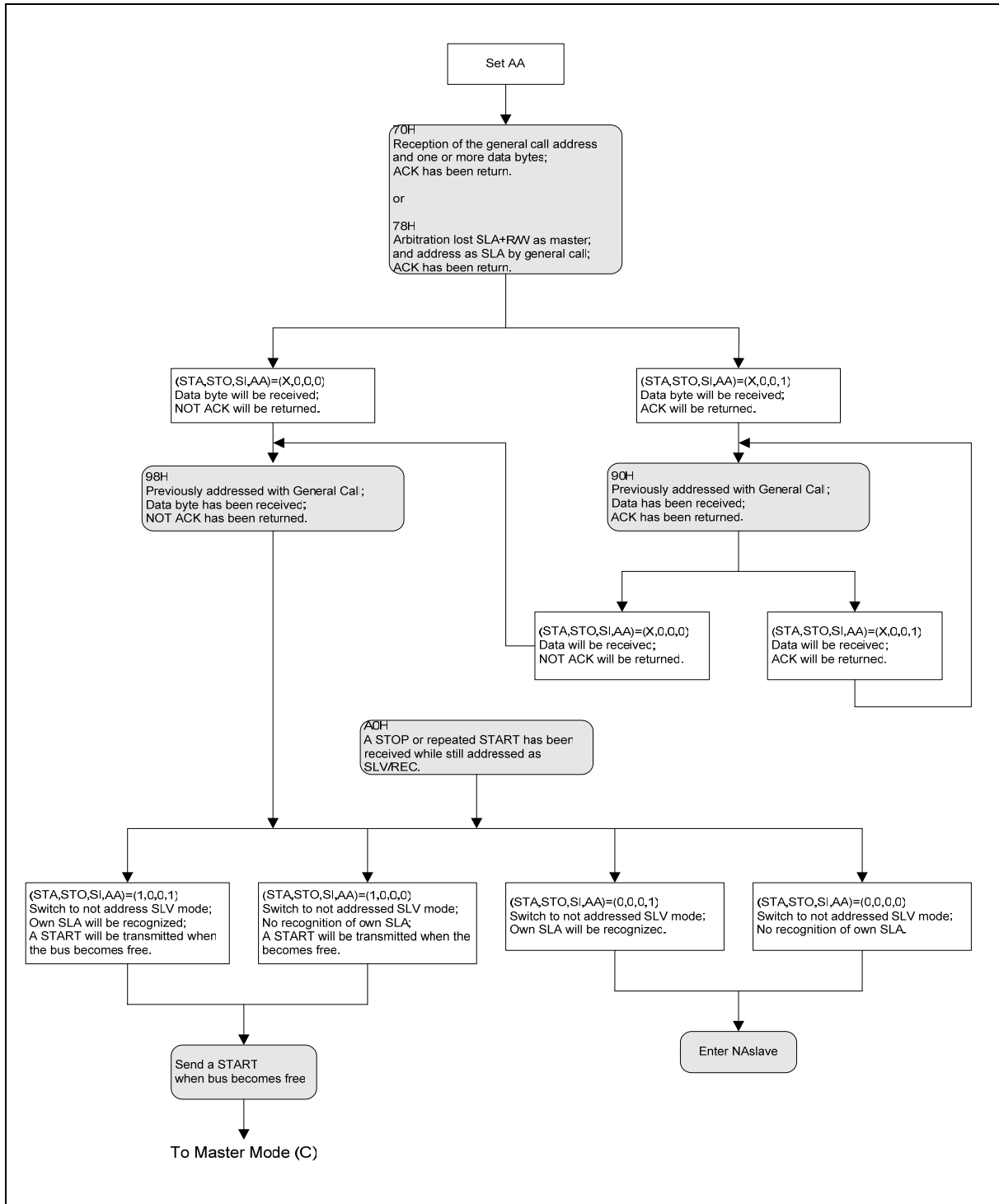
Figure 24-8: GC Mode
