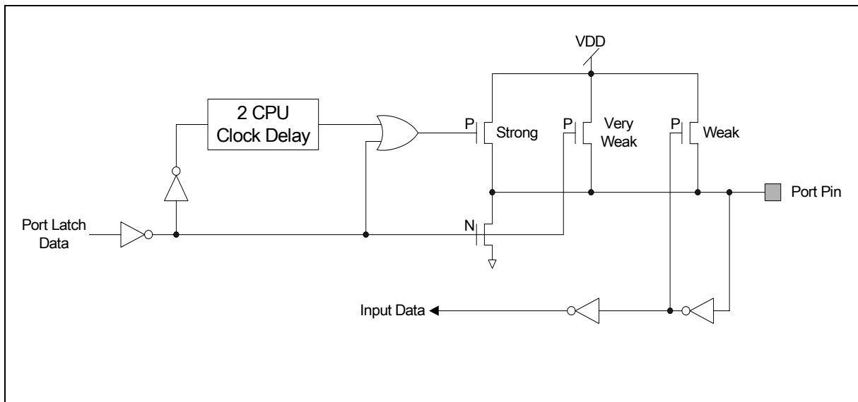
Figure 20-2: Quasi-Bidirectional Output
