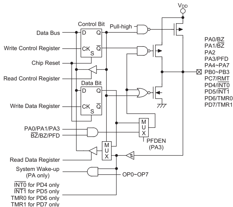
Input/Output Ports
