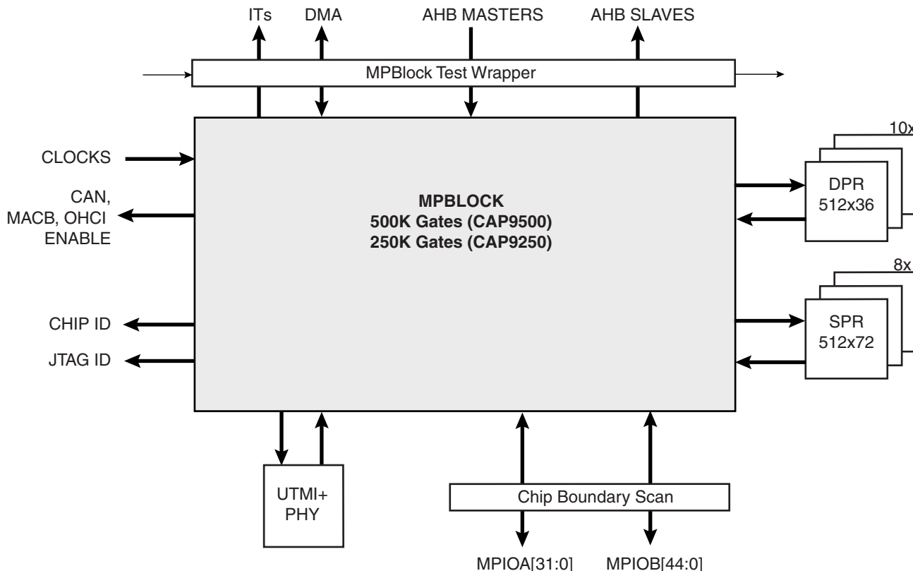
Figure 11-1. MPBlock Connectivity
