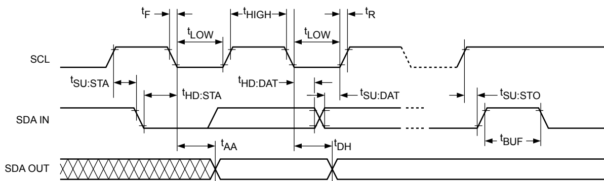
Figure 6. Bus Timing
