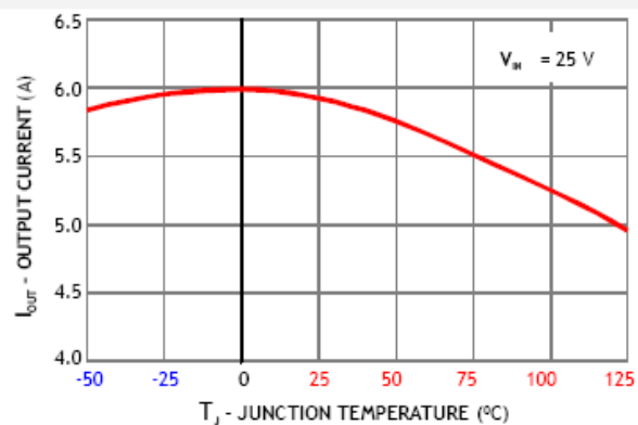
CURRENT LIMIT
