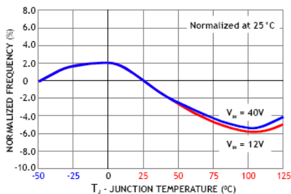
OSCILLATOR FREQUENCY
