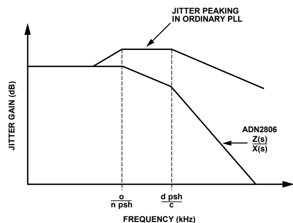
Figure 14. Jitter Response vs. Conventional PLL
