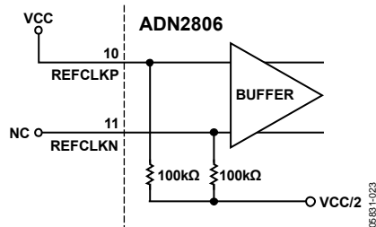
Figure 18. No REFCLK Configuration
