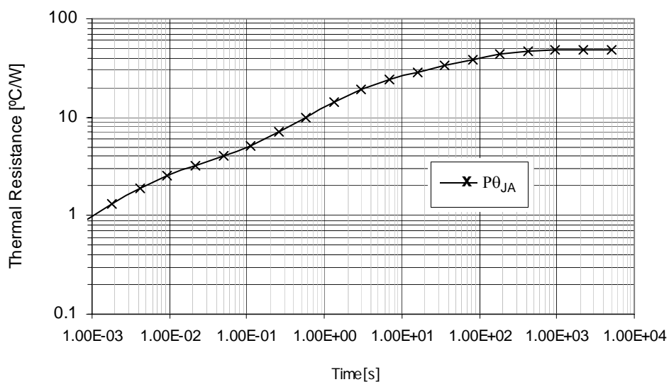
Figure 26. Transient Pin Resistance P\theta_{JA} Device on Thermal Test Board Area A = 600 ( \text{mm}^2 )
