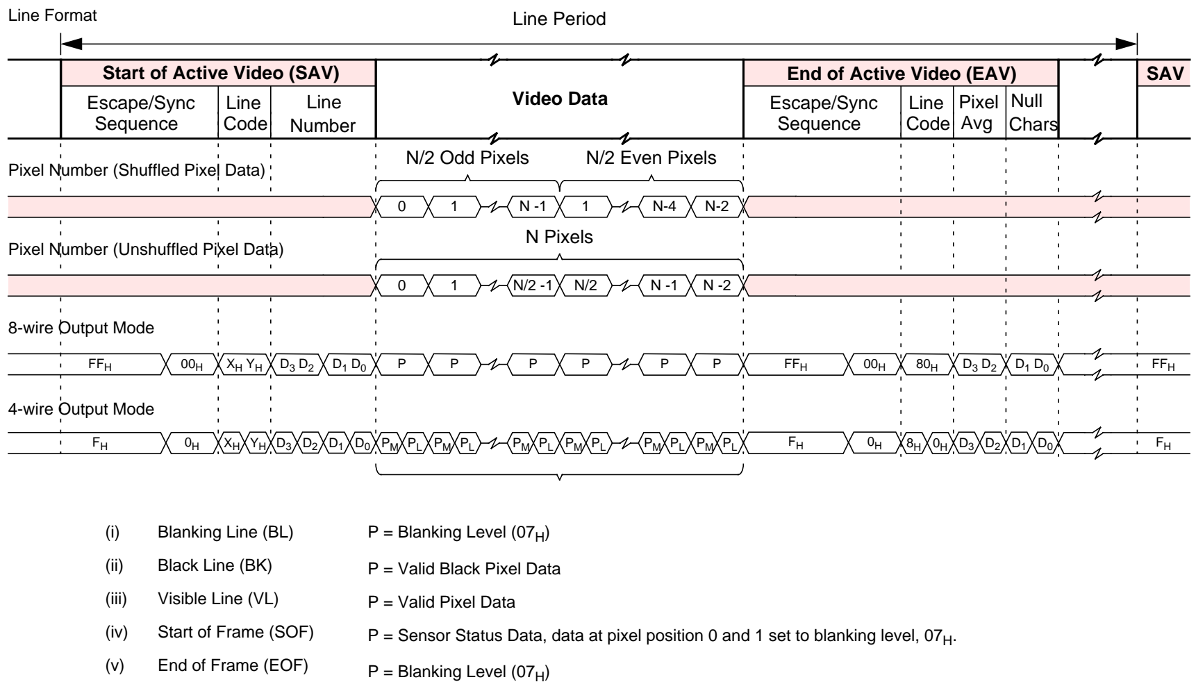
Figure 26 : Line Data Format.
