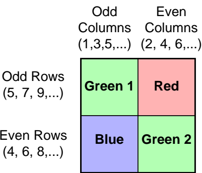
Figure 2 : Bayer Colourisation Pattern (VV6410 only)
