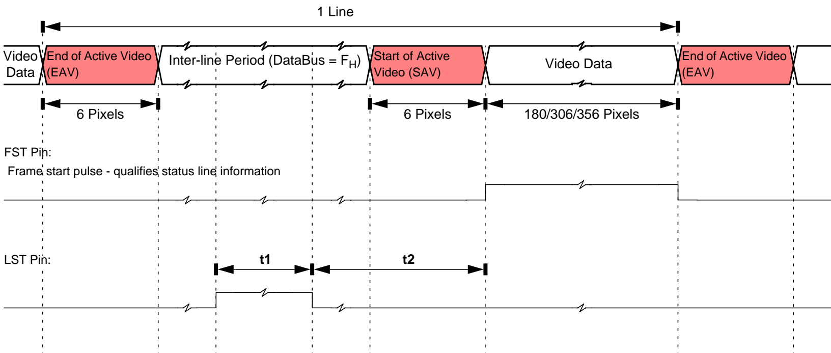
Figure 33 : Line Level Timings for FST and LST.
