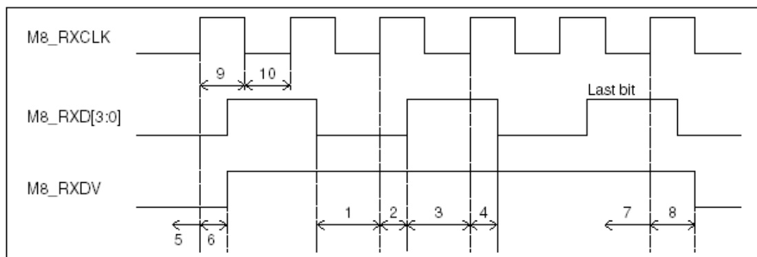
Figure 8 - Receive Timing
