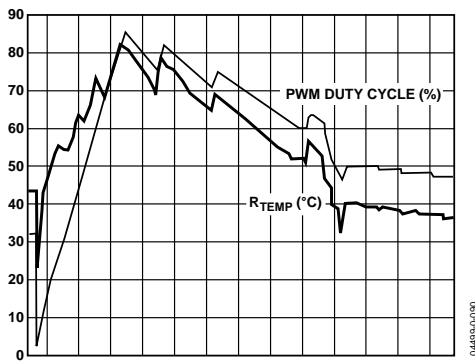
Figure 84. How Fan Reacts to Temperature Variation in Enhanced Acoustics Mode
