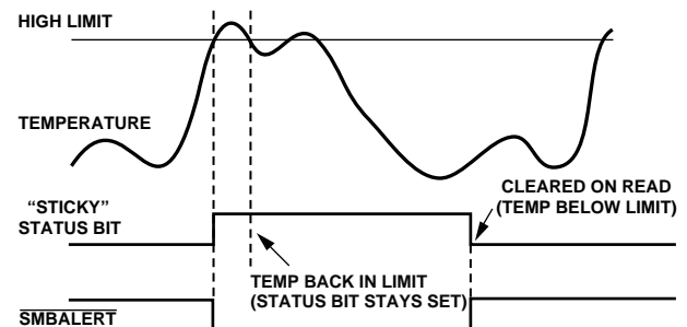
Figure 28. \overline{\text{SMBALERT}} and Status Bit Behavior
