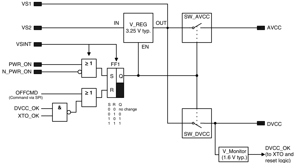
Figure 10-1. Power Supply
