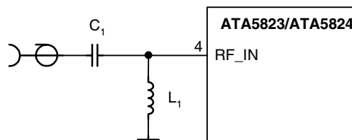
Figure 7-1. Input Matching to 50Ω
