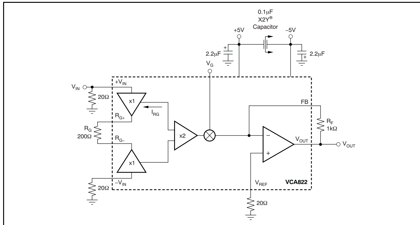
Figure 77. DC-Coupled, A_{V\text{MAX}} = +10\text{V/V} , Bipolar Supply Specification and Test Circuit
