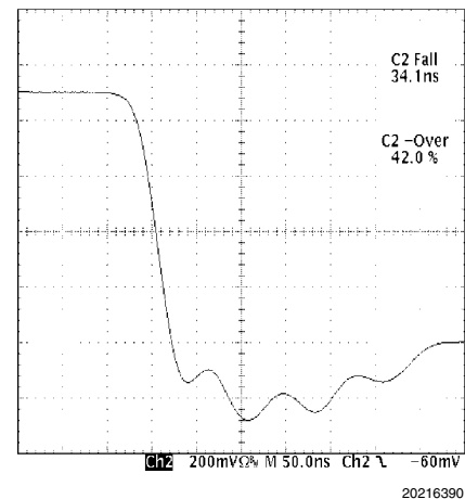
FIGURE 18. Fall Time
