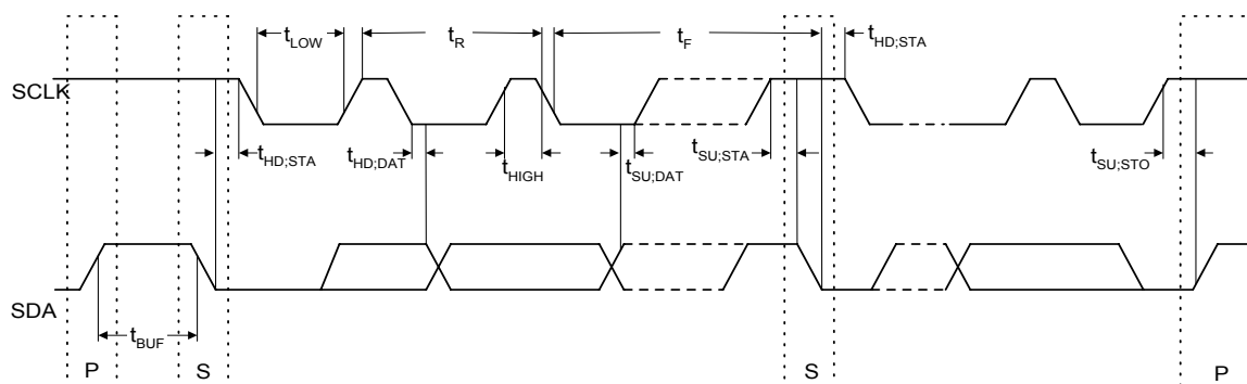
Figure 9.4 SMBus Timing
