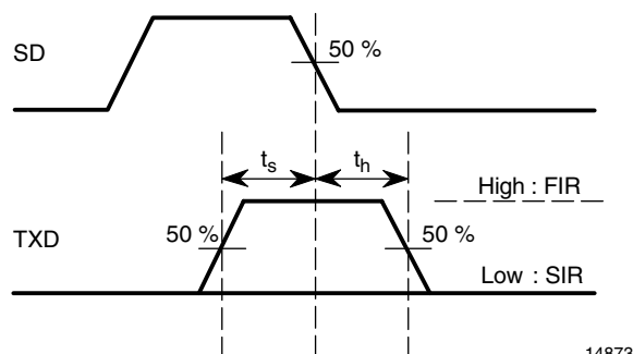
Figure 3. Mode Switching Timing Diagram
