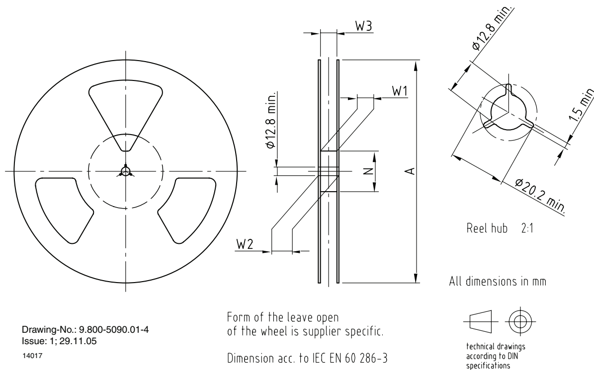
Figure 10. Reel dimensions, tolerance \pm 0.2 \text{ mm} , if not otherwise mentioned
