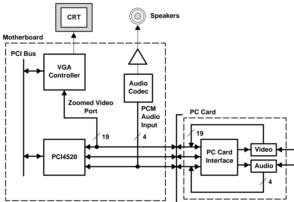
Figure 3–3. Zoomed Video Implementation Using the PCI4520 Device
