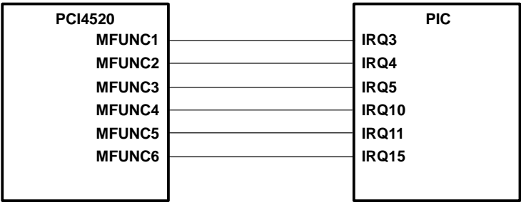
Figure 3–12. IRQ Implementation
