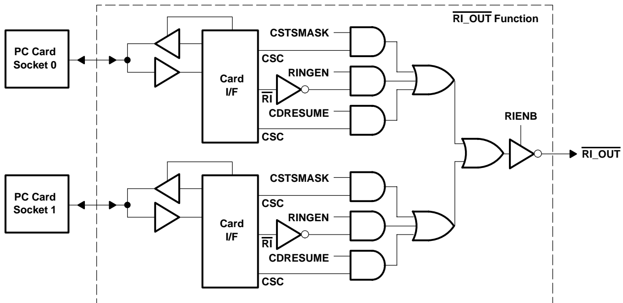
Figure 3-14. \overline{\text{RI\_OUT}} Functional Diagram
