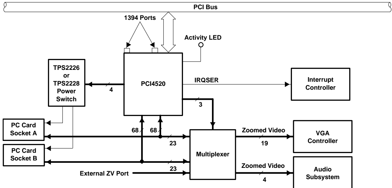
Figure 3–1. PCI4520 System Block Diagram
