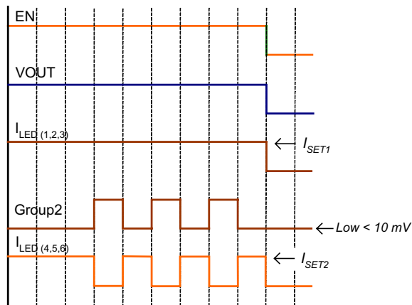
Figure 8. PWM Signal Dimming
