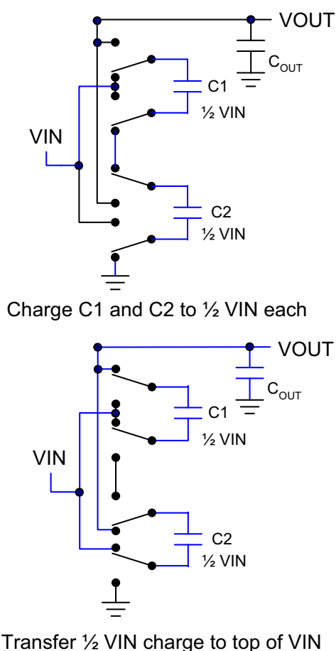
Figure 1. Switch Operation
