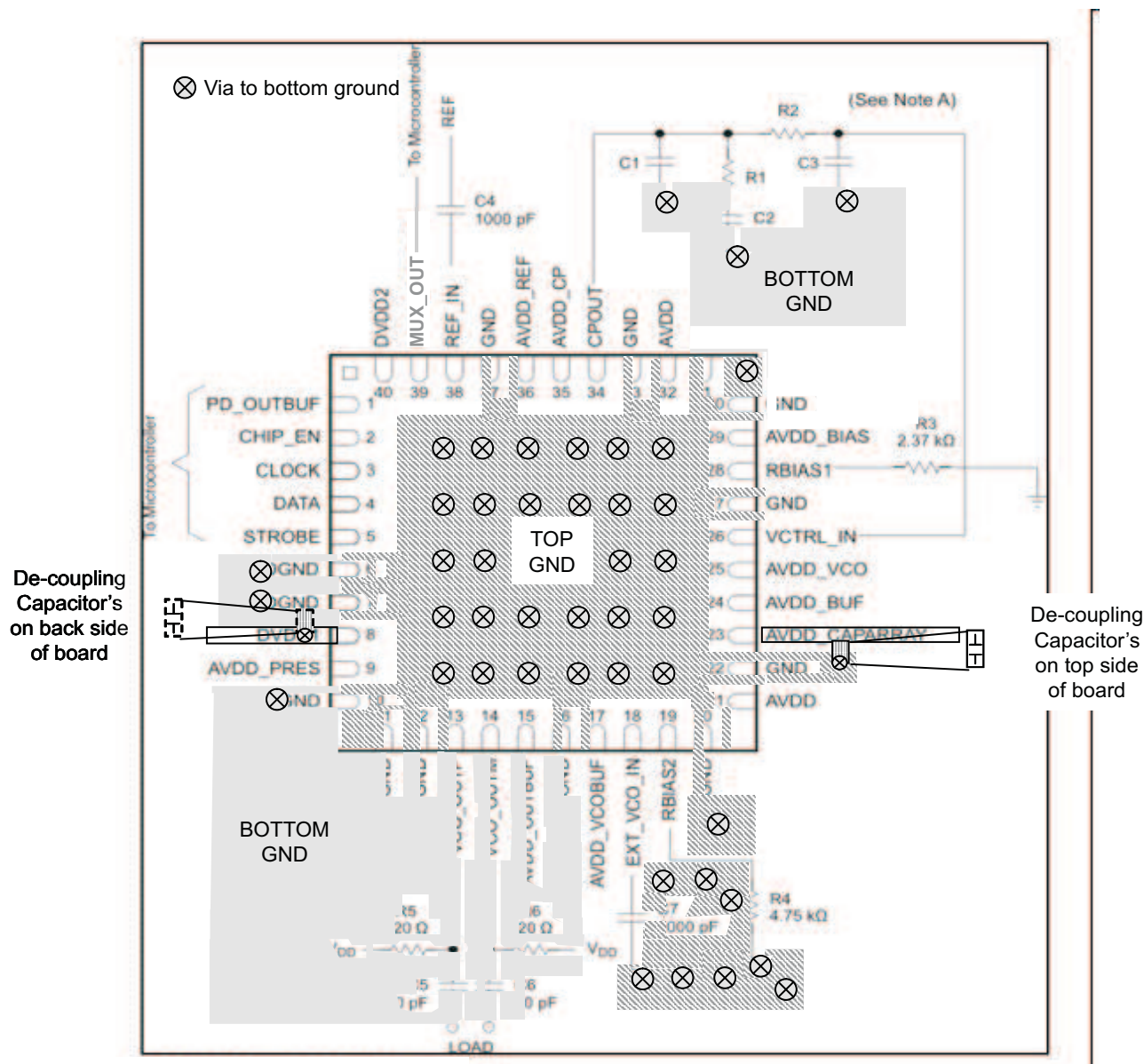
Figure 80. TRF3761 Layout
