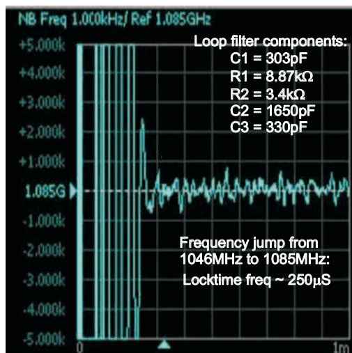
Figure 79. Frequency Locktime
