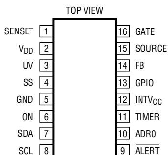
GN PACKAGE 16-LEAD PLASTIC TSSOP T_{JMAX} = 125^{\circ}C , \theta_{JA} = 130^{\circ}C/W
