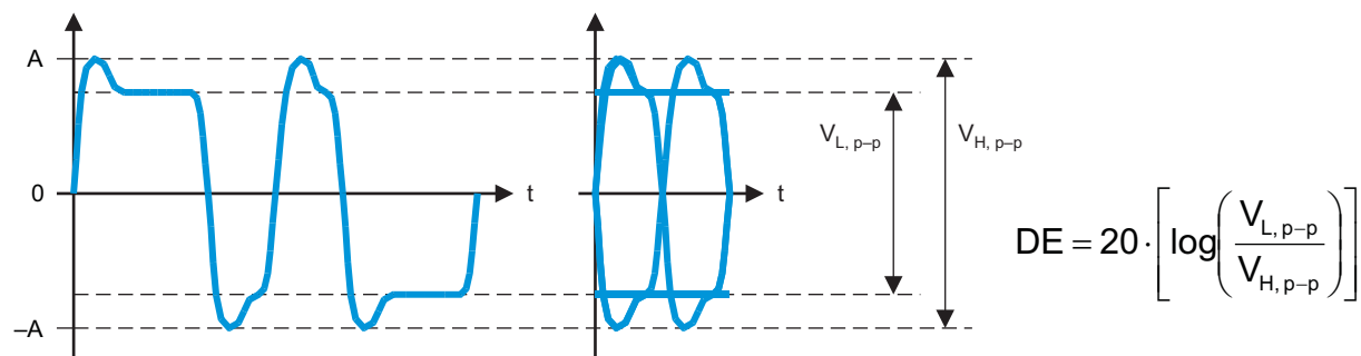
Figure 3. Output De-emphasis
