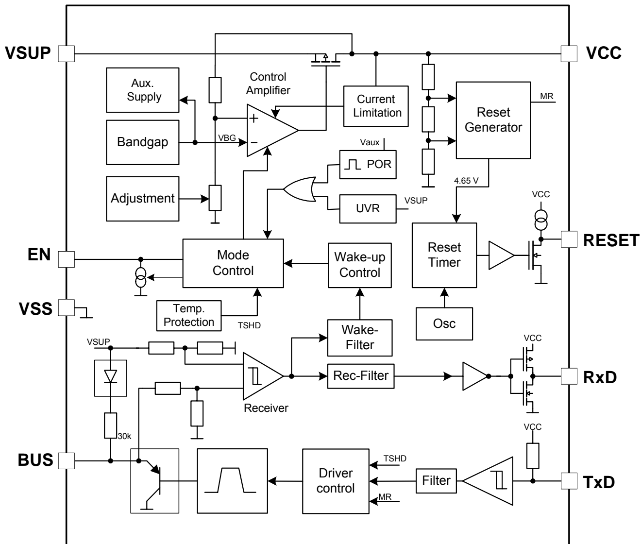
Figure 1 - Block diagram
