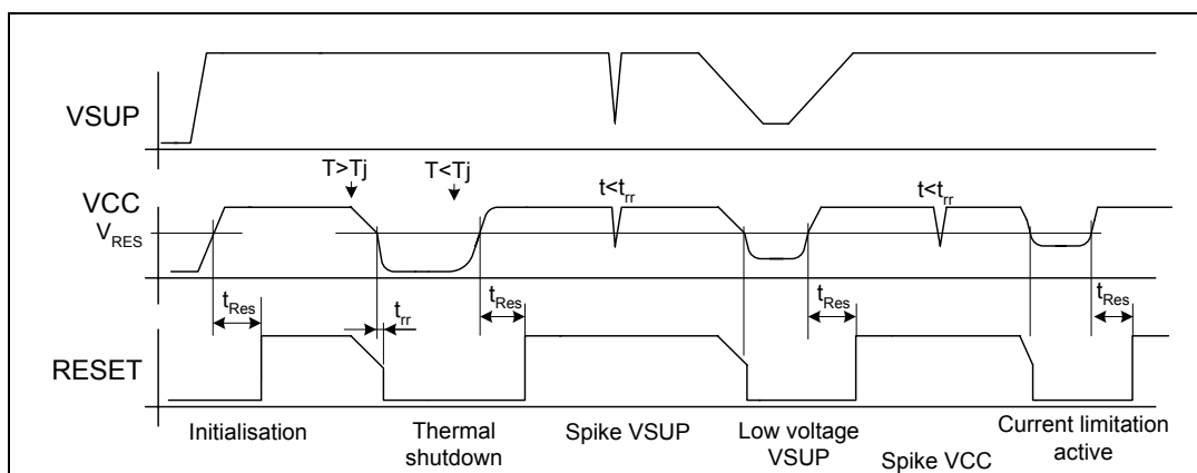
Figure 16 - Reset behaviour
