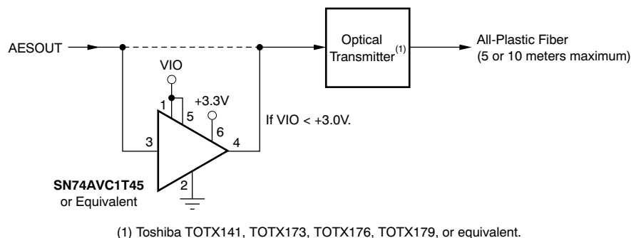
Figure 90. Interfacing to an Optical Transmitter Module
