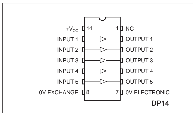
Figure 1: Pin connections (viewed from underside)
