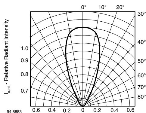
Figure 8. Relative Radiant Intensity vs. Angular Displacement
