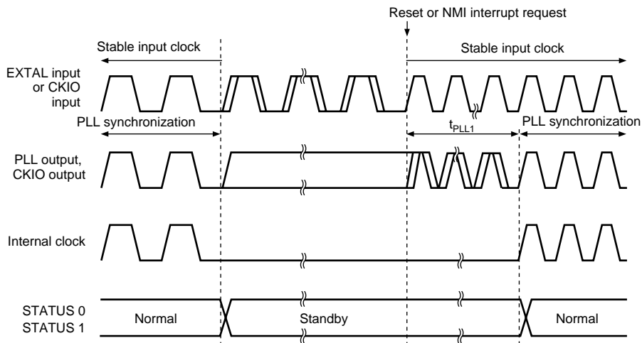
Figure 24.8 PLL Synchronization Settling Time by Reset or NMI at the returning from Standby mode (Return by Reset or NMI)
