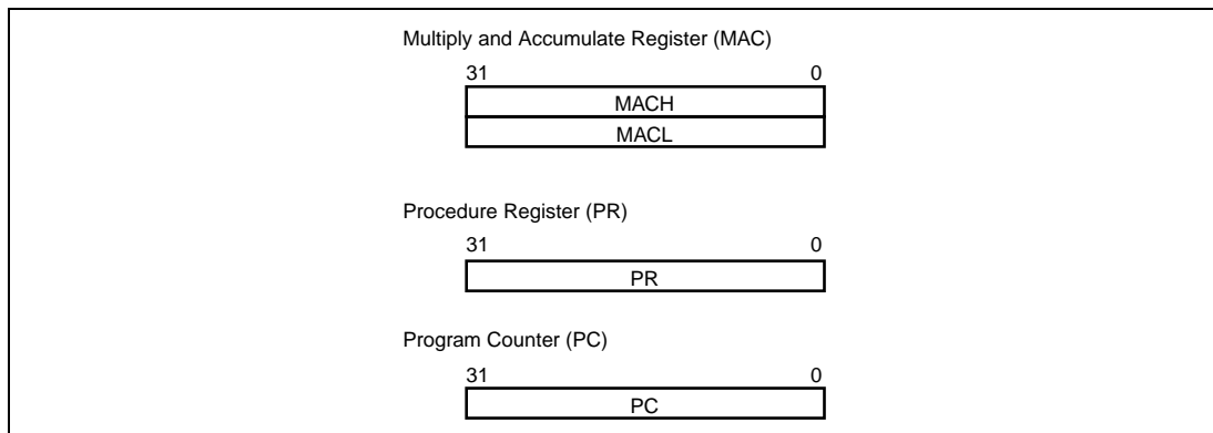
Figure 2.3 System Registers
