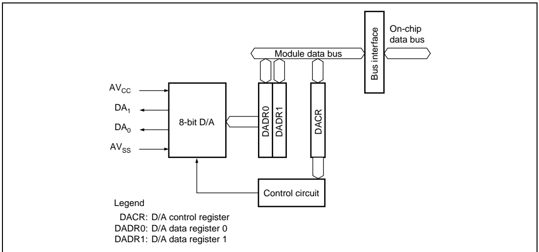
Figure 20.1 D/A Converter Block Diagram
