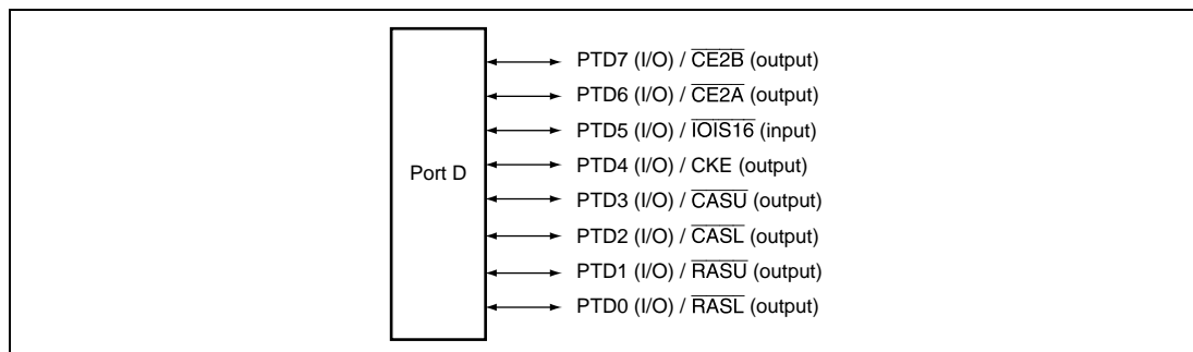
Figure 18.4 Port D
