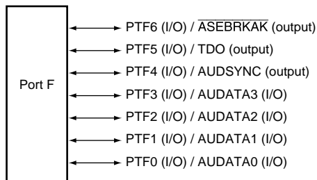
Figure 18.6 Port F
