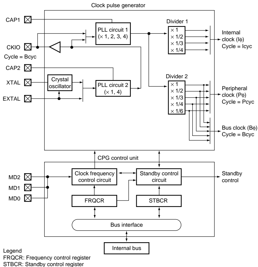
Figure 10.1 Block Diagram of Clock Pulse Generator
