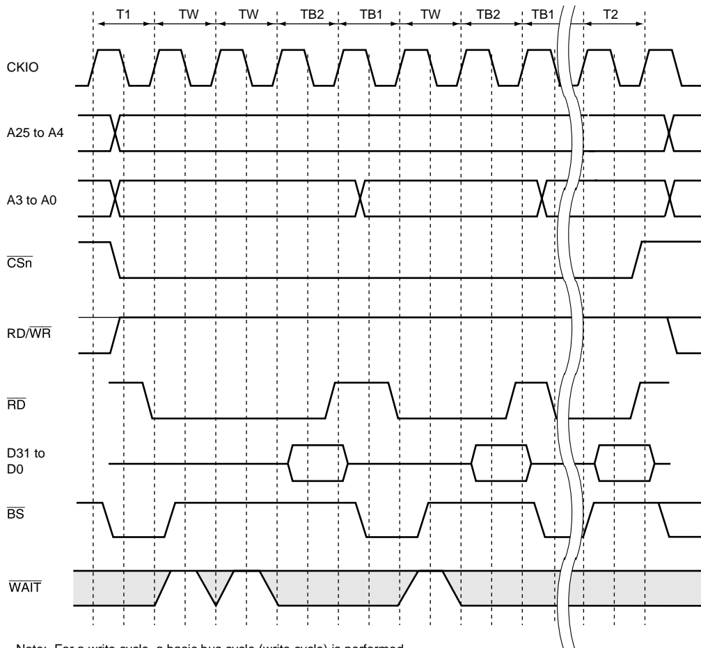
Figure 8.28 Burst ROM Wait Access Timing
