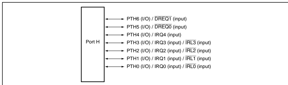
Figure 18.8 Port H
