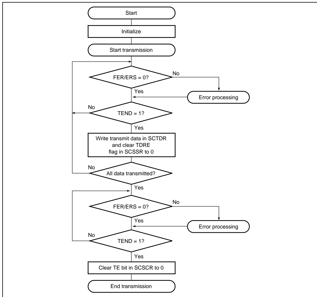
Figure 15.6 Transmission Flowchart
