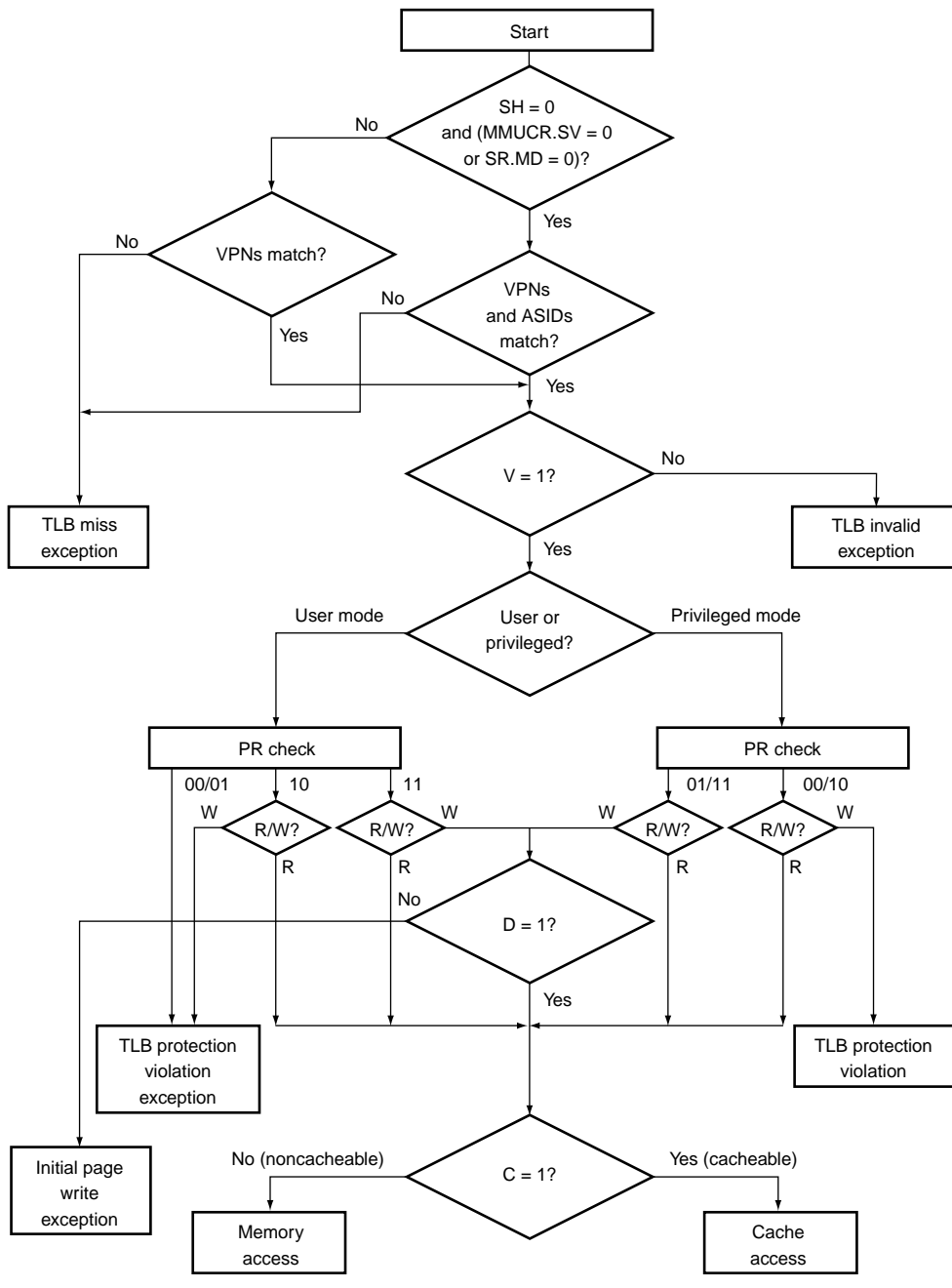
Figure 3.10 MMU Exception Generation Flowchart
