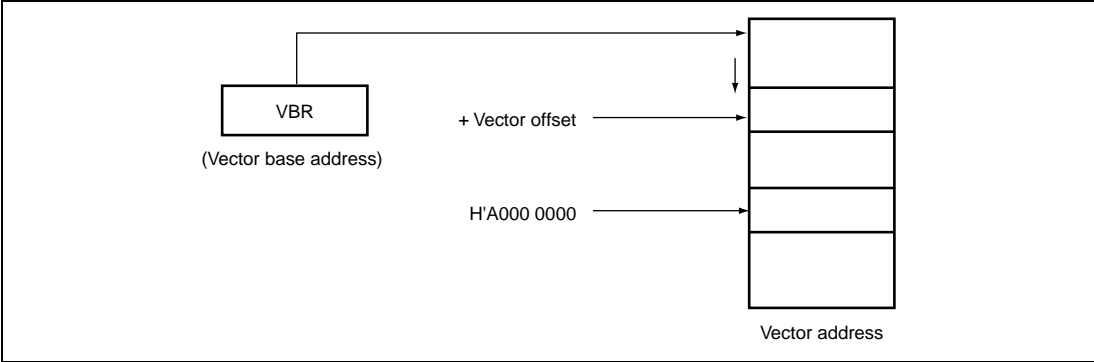
Figure 4.1 Vector Addresses
