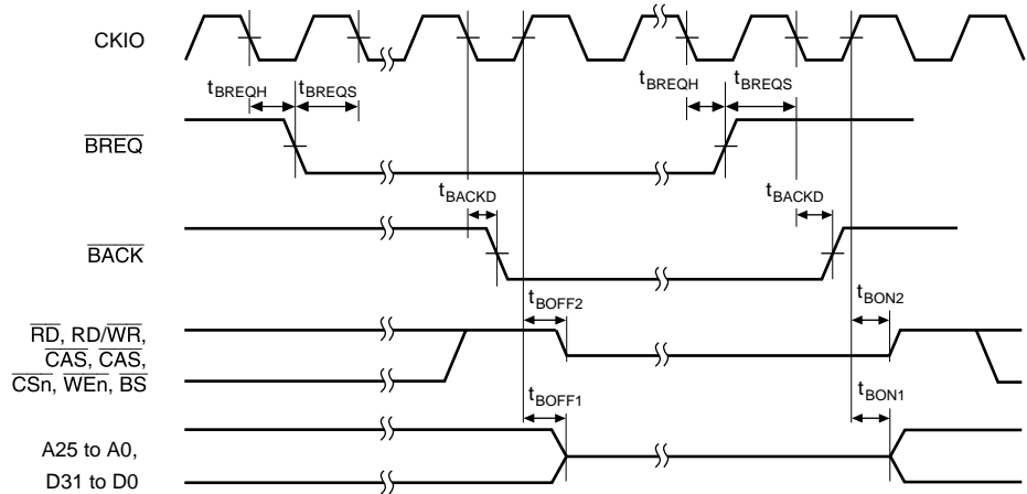
Figure 24.14 Bus Release Timing
