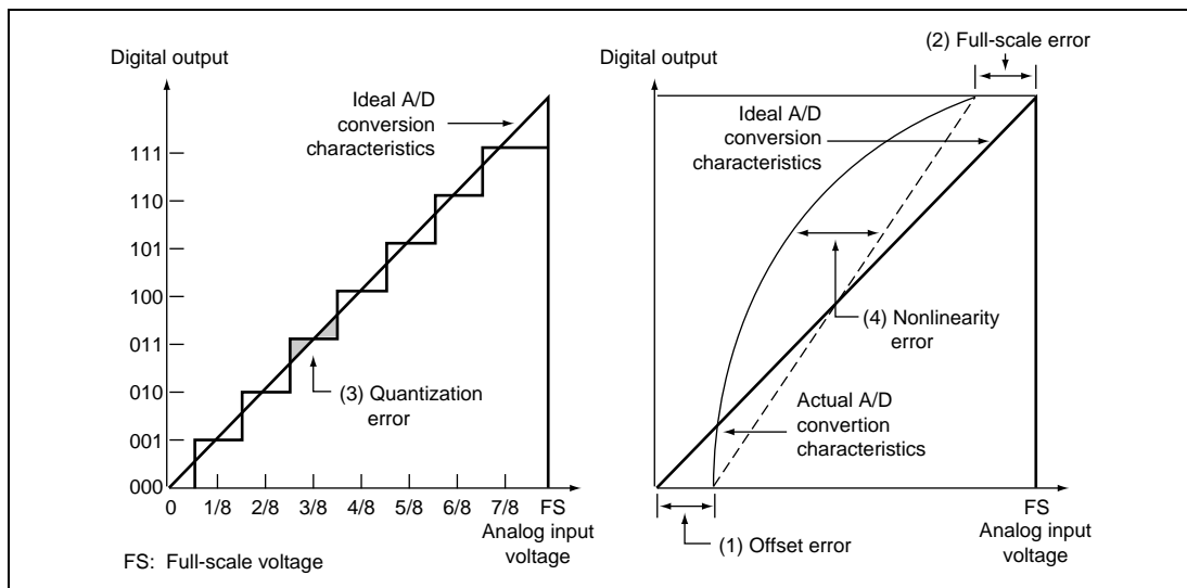
Figure 19.10 Definitions of A/D Conversion Accuracy
