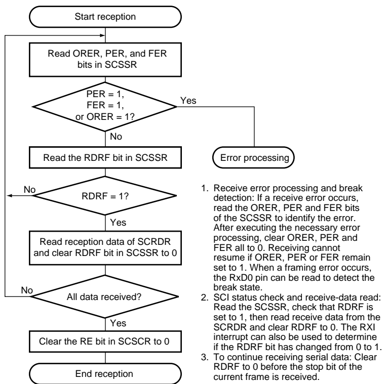
Figure 14.10 Sample Flowchart for Receiving Serial Data
