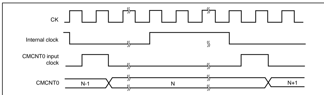
Figure 9.28 Count Timing
