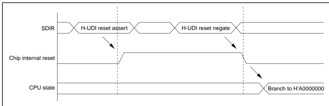
Figure 21.3 H-UDI Reset
