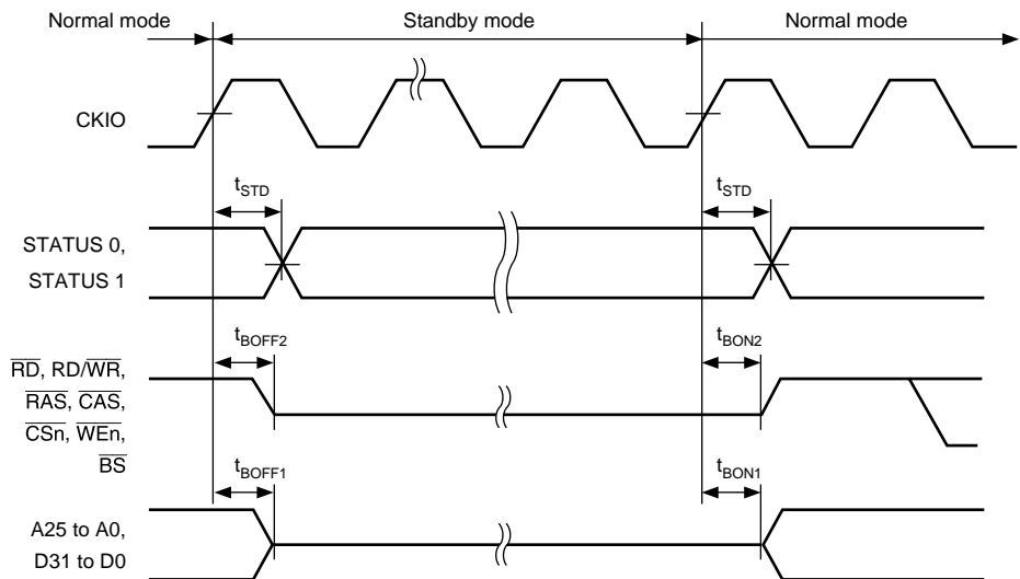
Figure 24.15 Pin Drive Timing at Standby
