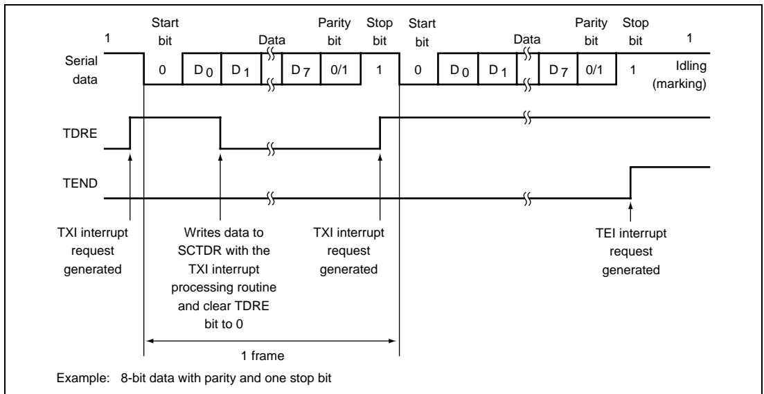
Figure 14.9 SCI Transmit Operation in Asynchronous Mode
