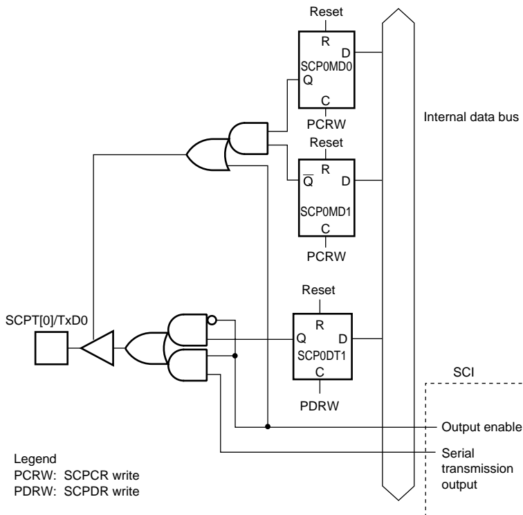
Figure 14.3 SCPT[0]/TxD0 Pin
