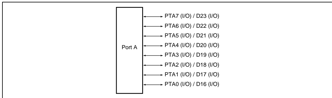
Figure 18.1 Port A
