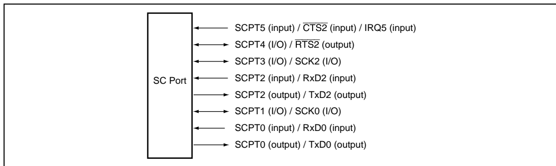
Figure 18.10 SC Port
