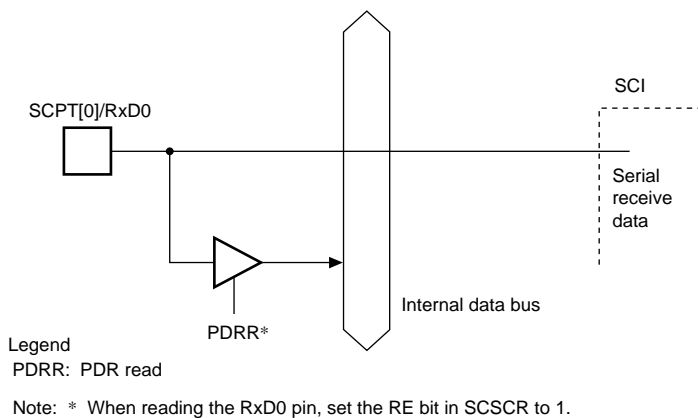
Figure 14.4 SCPT[0]/RxD0 Pin
