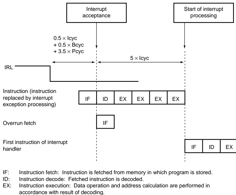
Figure 6.4 Example of Pipeline Operations when IRL Interrupt is Accepted
