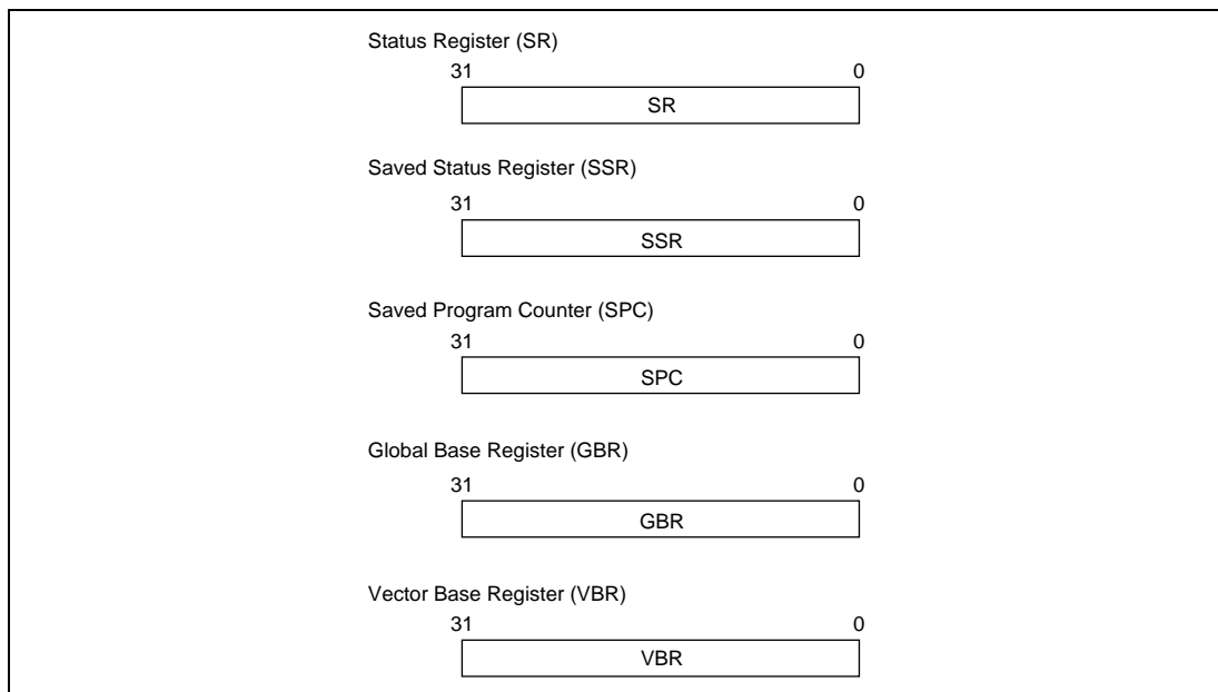
Figure 2.4 Control Registers
