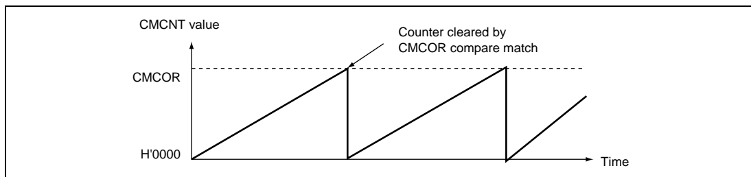
Figure 9.27 Counter Operation
