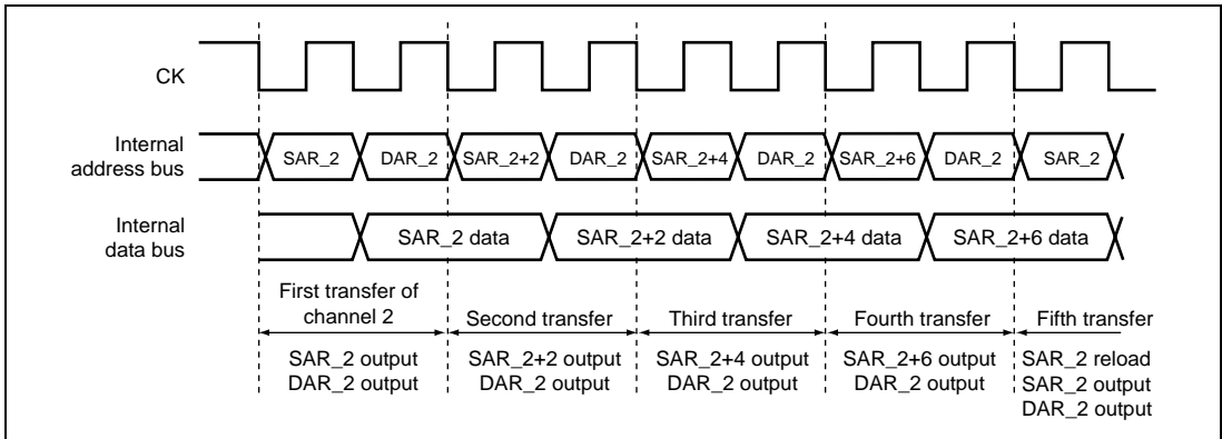
Figure 9.25 Timing Chart of Source Address Reload Function
