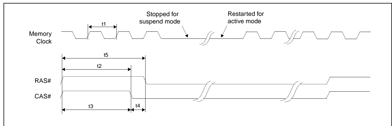
Figure 7-16: FPM-DRAM CBR Self-Refresh Timing
