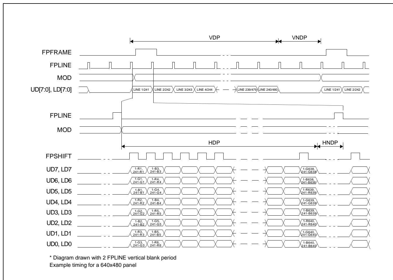
Figure 7-35: Dual Color 16-Bit Panel Timing
