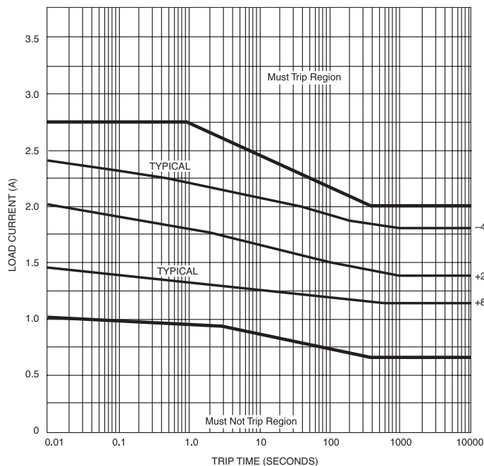
TYPICAL TRIPP CURRENT VS. TIME FIGURE 4
