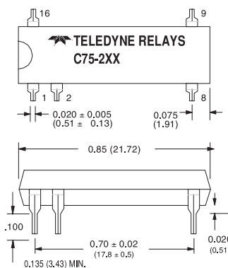
DIMENSIONS ARE IN INCHES (MILLIMETERS) Tolerances ± 0.015 (0.38) unless specified.
