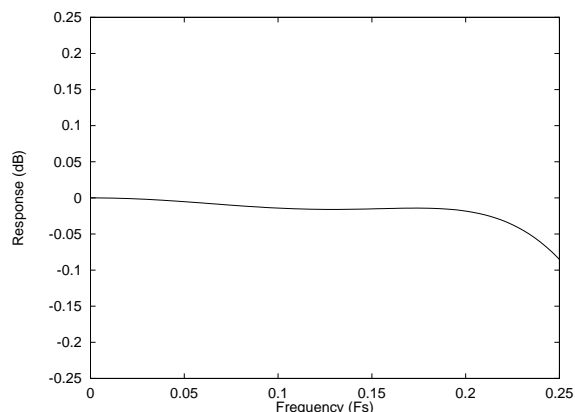
Figure 42 ADC Digital Filter Ripple – Type 2
