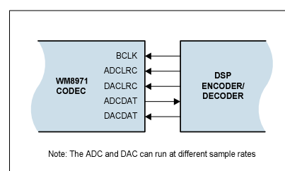
Figure 18 Slave Mode
