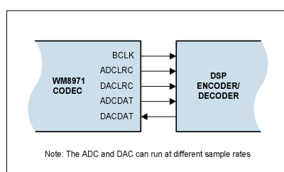
Figure 17 Master Mode
