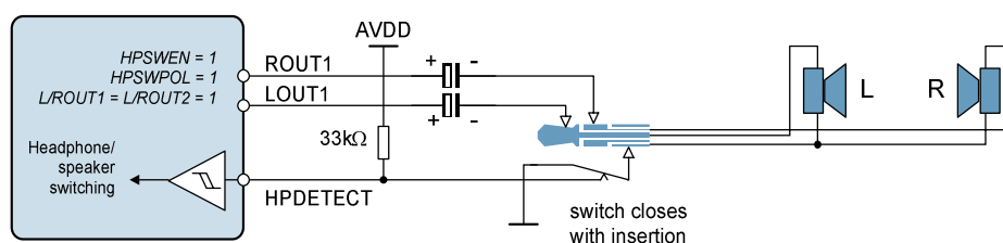
Figure 13 Example Headset Detection Circuit Using Normally-Closed Switch
