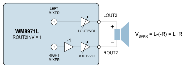
Figure 15 Speaker Output Connection
