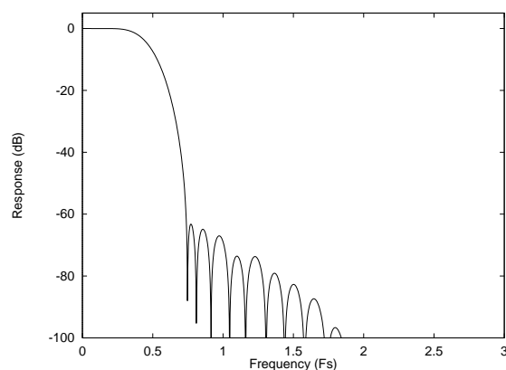
Figure 43 ADC Digital Filter Frequency Response – Type 2
