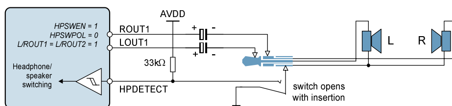
Figure 12 Example Headset Detection Circuit Using Normally-Open Switch
