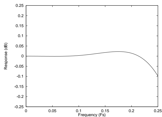
Figure 44 ADC Digital Filter Ripple – Type 3
