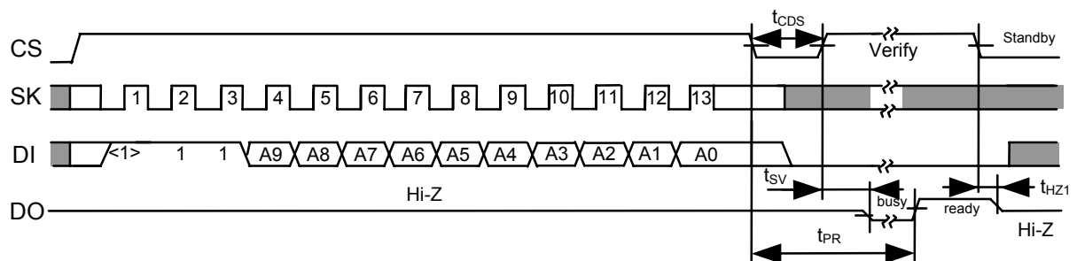
Figure 7 Data Erase Timing
