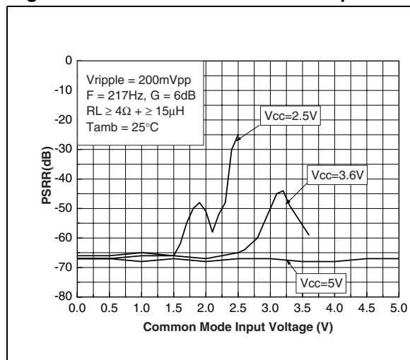
Figure 20. PSRR vs. common mode input voltage
