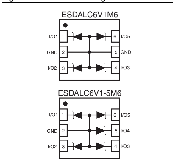
Figure 1. Functional diagram
